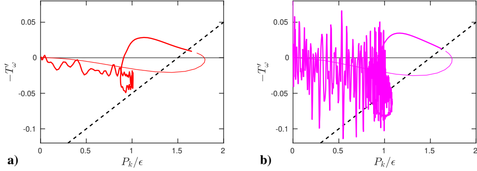
Fig. B2 Test of the \omega equation of the k - \omega model in channel flows. The continuous curve shows the opposite of the normalized transport term -T'_\omega for the DNS of [7] at Re_\tau = 543 (a), 5186 (b). The thin (resp. thick) curve corresponds to the inner region y^+ < 15 (resp. outer region y^+ > 15 ). The dashed line shows the standard model \sigma_\omega (\beta^* \gamma P_k/\epsilon - \beta) .
