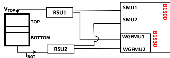
Fig.3. Measurement setup a probe and an Analyzer B1500 of Keysight Technologies brand.
