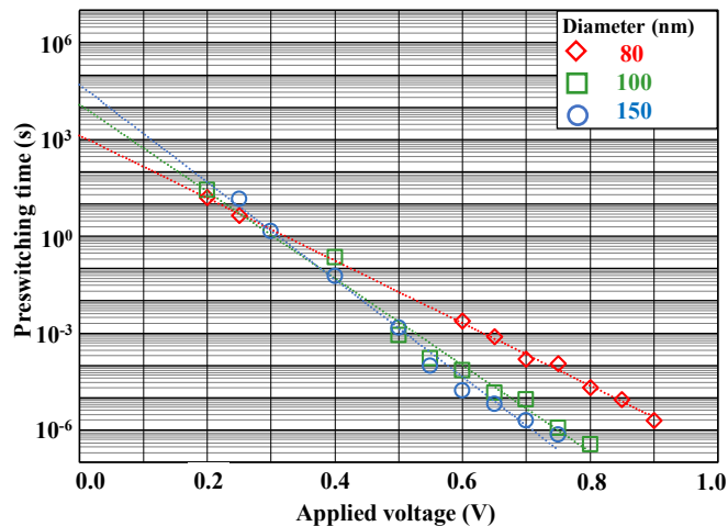
Fig. 7. The average over 30 measurements of the preswitching time for each of the 3 cells of diameter 80, 100 and 150 nm.
