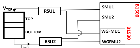
Fig.3. Measurement setup a probe and an Analyzer B1500 of Keysight Technologies brand.
