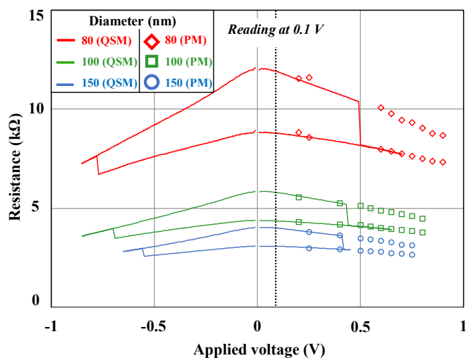
Fig. 6. Resistance as a function of the applied voltage in quasi-static mode (Fig. 4), as well as their corresponding average pulse mode resistances over 30 measurements.
