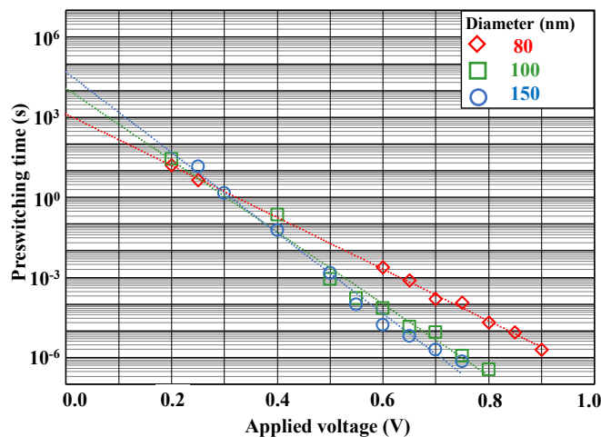
Fig. 7. The average over 30 measurements of the preswitching time for each of the 3 cells of diameter 80, 100 and 150 nm.
