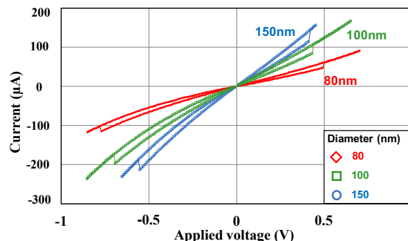
Fig. 4. Quasi-static measured current ( I_{BOT} ) as a function of the applied voltage ( V_{TOP} ) for cells with diameters 80 nm, 100 nm and 150 nm.
