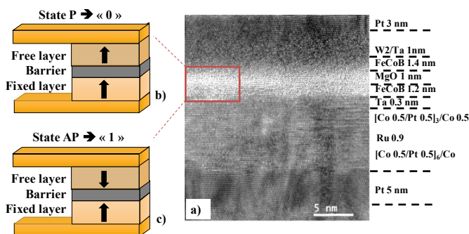
Fig. 1. (a) HRTEM images of p-MTJ of STT-MRAM stack [3], (b) P state and (c) AP state configurations.
