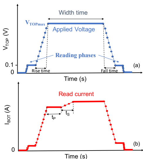
Fig. 2. (a) Applied bias voltage pattern showing the rise, width and fall times and the reading phase at 0.1 V, (b) read current and the extraction of the preswitching ( t_p ) and the switching ( t_s ) times.
