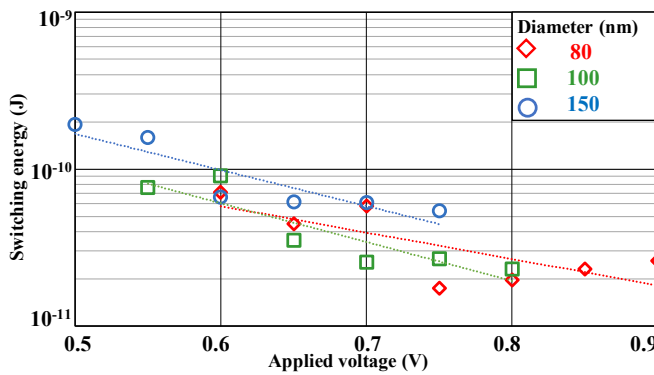
Fig. 10. Average over 30 measurements of the switching energy for each of the three cell diameters 80, 100 and 150 nm.
