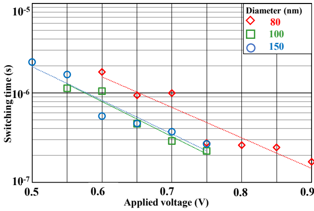
Fig. 8. The average over 30 measurements of the switching time for each of the 3 cells of diameter 80, 100 and 150 nm.
