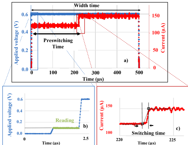
Fig. 5. (a) Experimental result showing applied voltage and measured current for VTOPmax = 0.6V, width time = 500µs, sampling time= 10 ns and the rise-fall time= 100 ns, as well as definition of preswitching time. (b) reading voltage and (c) switching time.
