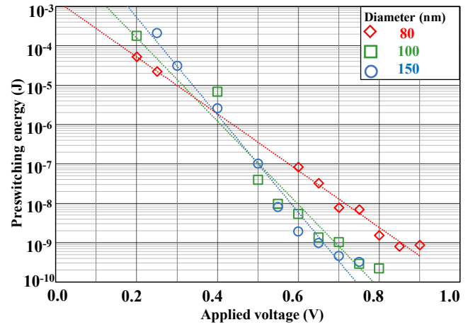
Fig. 9. Average over 30 measurements of the preswitching energy for each of the three cell diameters 80, 100 and 150 nm.
