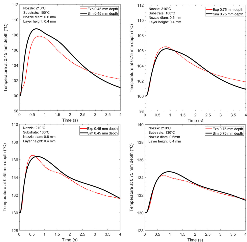
FIGURE 10 Influence of thermocouple depth and substrate temperature on the predicted temperature rise in the substrate for a nozzle set at 210°C. The black line corresponds to the predicted temperature and the red lines to the average
