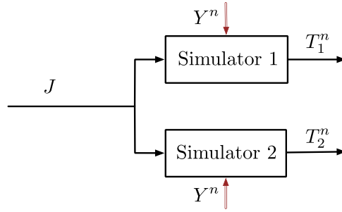
FIG. 2. A simulation problem with side information. We require that d_{\text{TV}} \left( P_{T_1^n T_2^n Y^n}; Q_{T_1 T_2 Y}^{\otimes n} \right) approach 0.
