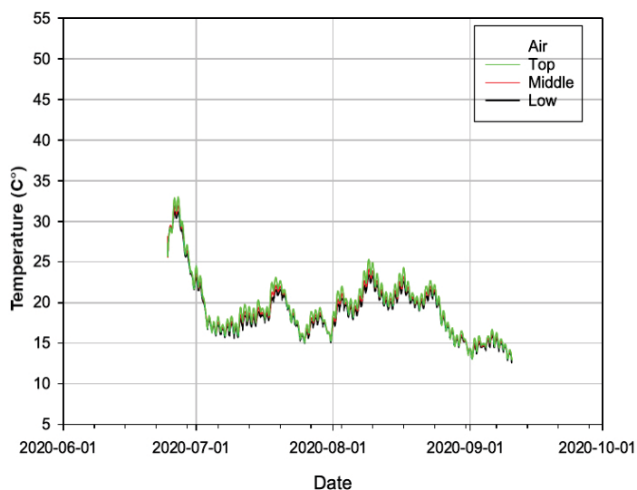
Fig. 2. Temperature of samples stabilized by 150 kg of binder per \text{m}^3 of the dredged soil collected from site B4
