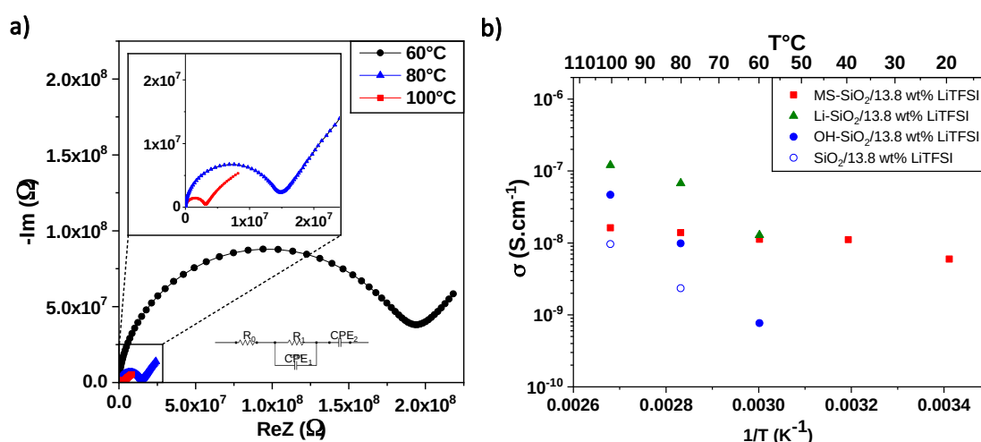
Figure 4: a) Nyquist diagrams performed at 60 °C, 80 °C, 100 °C of OH-SiO 2 /13.8 wt% in a blocking electrode/solid electrolyte/blocking electrode system and corresponding equivalent circuit. Nyquist diagrams for other samples are available in SI (Figure S3). b) Temperature dependencies of the ionic conductivity of MS-SiO 2 , Li-SiO 2 , OH-SiO 2 and SiO 2 /13.8 wt% LiTFSI, measured between 20 °C and 100 °C.
