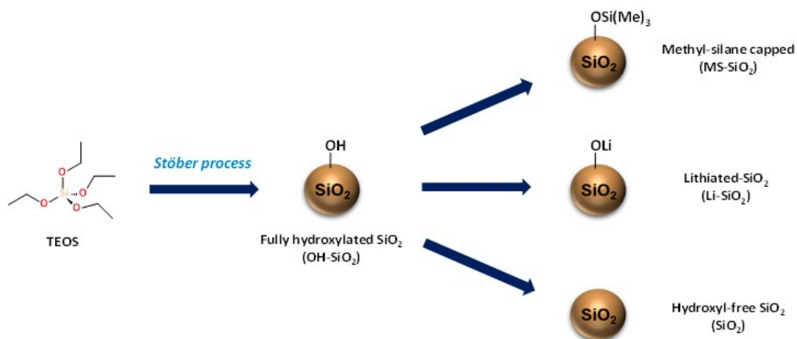
Figure 2: Surface modifications of hydroxylated SiO 2 NPs (OH-SiO 2 ) by surface capping with HMDS (MS-SiO 2 ), Lithiation (Li-SiO 2 ) and hydroxyl-free (SiO 2 ).
