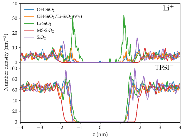
Figure 6: Number density profiles of \text{Li}^+ and \text{TFSI}^- at 350 K, along the axis perpendicular to the silica surface. The zero-density region of the curves corresponds to the position of the silica slab.
