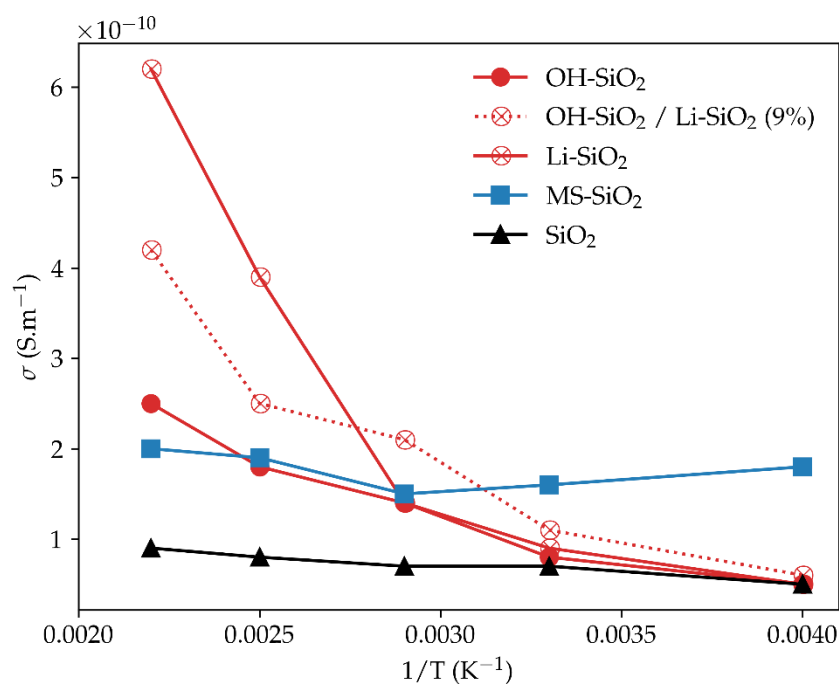
Figure 8: Static conductivities obtained using Einstein-Helfand fitting.
