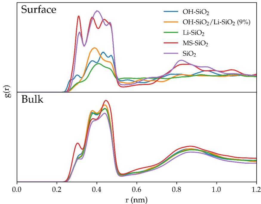
Figure 7: Radial distribution functions at 350 K between a Li cation and the nitrogen atom of the TFSI anion, obtained in the vicinity of the silica surface and in bulk solvent.
