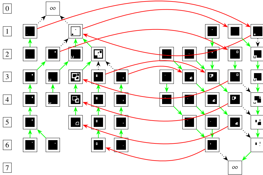
Fig. 2. Tree of valued shapes of the image \mathcal{F} (Figure 1(a)). The valued connected components are depicted by squares ( \mathcal{E}^\circ on the left side; \mathcal{E}^\bullet on the right side) and are positioned with respect to the threshold value v (see on left), from 0 (top) to 7 (bottom). Red and green arrows correspond to the \leq_{\mathcal{E}} relation. Green and black dotted arrows correspond to the <^{\psi} relation. Red arrows are a subset of the <^{\psi} relation, not fully depicted for the sake of readability.
