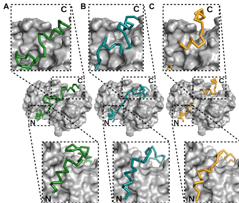
FIGURE 5 | Different modes of binding of p53 TAD to S100A4. (A, B) The two best models built, using NMR data (Dudás et al., 2020), and (C) X-ray crystal structure of the p53 TAD 17–56 –S100A4 complex (Ecsédi et al., 2020). p53 is shown as alpha-carbon traces in different colors, while S100A4 is shown as surface representations in gray. The labels N and C mark the locations of the N- and C-termini of the p53 peptide. The binding of the N-terminus is nearly identical in these three cases, but the C-terminus and the linker connecting the ordered regions differ, showing the different binding modes of p53. In the crystal structure determination, parts of the linker were not visible, indicative of its flexibility.
