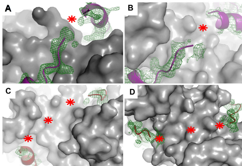
FIGURE 4 | Electron density maps of flexible regions in S100 complexes indicating fuzziness. Structures of (A) p53 TAD 17–56 –S100P (PDB: 7NMI), (B) p53 TAD 17–56 –S100A4 (PDB: 6T58) (Ecsédi et al., 2020), (C) RSK1 683–735 –S100B in one crystal form (PDB: 5CSN), and (D) RSK1 683–735 –S100B (PDB: 5CSJ) in another crystal form (Gógl et al., 2016). S100 proteins are displayed as gray surface representations and their partners as deep purple (p53 TAD 17–56 ) and red (RSK1 683–735 ) ribbons. The green meshes around the partner peptides are simulated annealing Fo–Fc omit maps (contoured at 2 \sigma ). Red asterisks show the tracks of flexible regions not appearing in the X-ray structures of these complexes.
