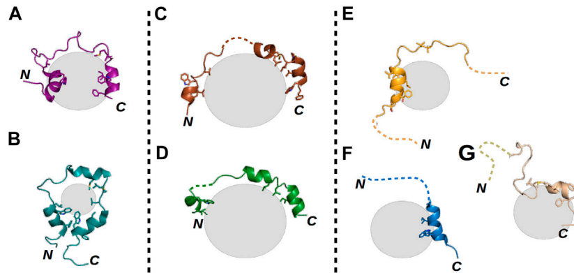
FIGURE 1 | Structural illustrations of various fuzzy interactions made by the p53 TAD. Gray spheres represent the different partner proteins, the labels N and C mark the locations of the termini of each p53 TAD chain, and dashed lines represent highly flexible disordered regions of the TAD in the respective complexes. (A) TAZ–p53 TAD 1–56 (PDB ID: 5HOU) (Krois et al., 2016) and (B) CRB–p53 TAD 13–61 (PDB ID: 2L14) (Lee et al., 2010) complexes represent polymorphic interactions, where nearly the whole TAD is bound with few alternative conformations. (C) S100P–p53 TAD 17–56 (PDB ID: 7NMI) and (D) S100A4–p53 TAD 17–56 (PDB ID: 6T58) (Ecsédi et al., 2020) complexes show the characteristics of clamp-like fuzzy interactions where the TAD is anchored at several binding points, while the linking regions remain flexible and appear in numerous conformations. Finally, (E) p300–p53 TAD 1–39 (PDB ID: 2K8F) (Feng et al., 2009), (F) TFIIH–p53 TAD 1–55 (PDB ID: 2GS0) (Di Lello et al., 2006), and (G) HMG box–p53 TAD 1–93 (PDB ID: 2LY4) (Rowell et al., 2012) complexes are good examples of flanking fuzzy interactions. Here, only a small portion of the TAD is binding the partner, while the sequences of the N- and C-termini remain disordered without any confinable structure.
