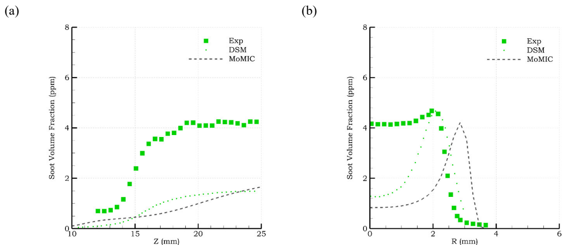
Figure 4. Soot volume fraction profiles along the flame centerline (a) and the radial direction at Z = 0.01896m (b). Exp, DSM and MOMIC correspond to, respectively, experimental data, discrete sectional method, and method of moments with interpolative closure.
