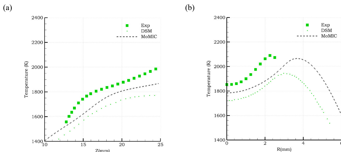
Figure 3. Temperature profiles along the flame centerline (a) and the radial direction at Z=0.01896\text{m} (b). Exp, DSM and MOMIC correspond to, respectively, experimental data, discrete sectional method, and method of moments with interpolative closure.
