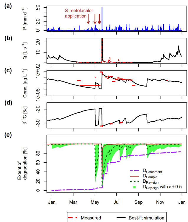
Figure 7. Measured (red lines) and modelled time series (black lines; best-fit simulation) for discharge (b), S-metolachlor concentrations (c; note the log-scaling), and \delta^{13}\text{C} values (d), as well as the extent of degradation as obtained by the Rayleigh equation ( D_{\text{Rayleigh}} , dotted green line; range of D_{\text{Rayleigh}} for \epsilon_C = -1.13 \pm 0.5\text{‰} , green area) and as known from the model for the sample ( D_{\text{Sample}} , solid brown line) and for the entire catchment ( D_{\text{Catchment}} , dashed purple line; e). Blue bars in (a) indicate daily precipitation and brown arrows indicate the dates of pesticide application.
