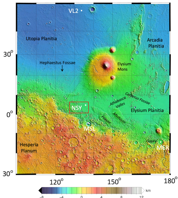
Figure 1. Locations of the InSight lander (NSY) close to the equator ( 4.502^\circ\text{N}/135.623^\circ\text{E} ), not far from the dichotomy boundary that separates, on Mars, the southern heavily cratered highlands from the northern lowlands (see color scale). The location of Hephæstus Fossae (see Figure 6) is also indicated. The map is a portion of the Mars Orbiter Laser Altimeter (MOLA) shaded topographic map of Mars (after Golombek et al. 2018).
