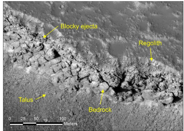
Figure 5. A portion of the exposed steep scarp of Hephaestus Fossae in southern Utopia Planitia (Golombek et al. 2018).
