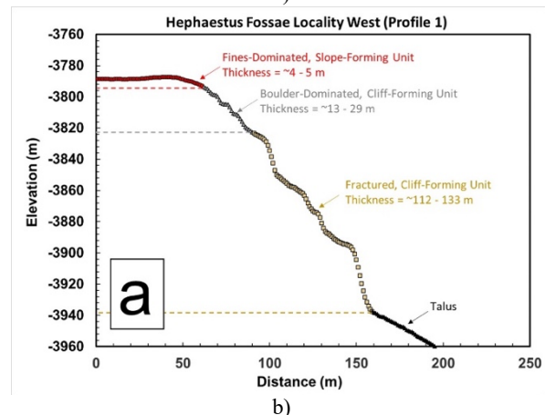
Figure 6. a) HiRISE image (ESP_052638_2020) of the Hephaestus Fossae exposure, a fracture ~900 km northwest of the InSight landing site; b) Slopes determined along profile 1 (Warner et al. 2022a, b).
