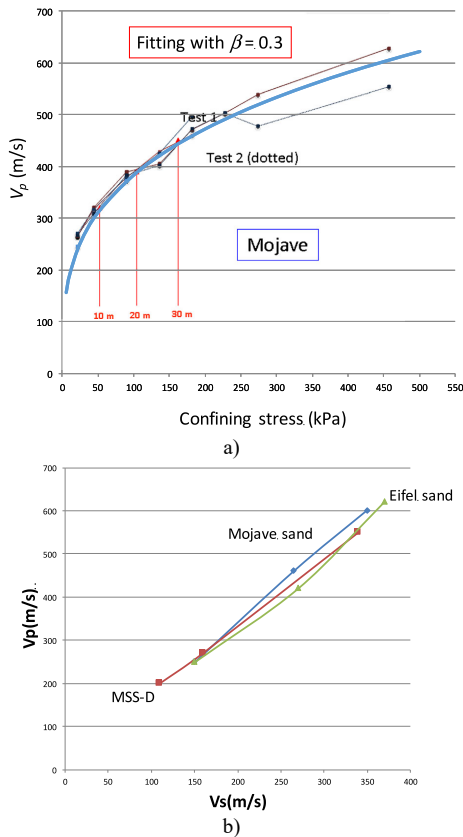
Figure 13. Bender elements measurements of velocity waves: a) changes in V_p with confining stress; b) linear relation between V_p and V_s for the three simulants investigated. A common value \nu = 0.22 is obtained for the three simulants tested (Delage et al. 2017).
