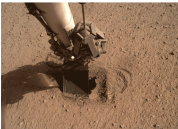
Figure 8. IDC photo showing the scoop of the Instrument Deployment Arm compressing the regolith, once the pit filled. The tether appears on the left side. The scoop width is 7.6 cm (image credit JPL/NASA).
