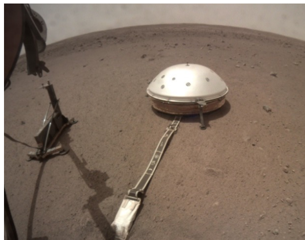
Figure 3. Photo taken from the Instrument Context Camera (ICC) showing the location of SEIS and of the \text{HP}^3 support structure, 1.18 meter apart from each other (image credit JPL/NASA).
