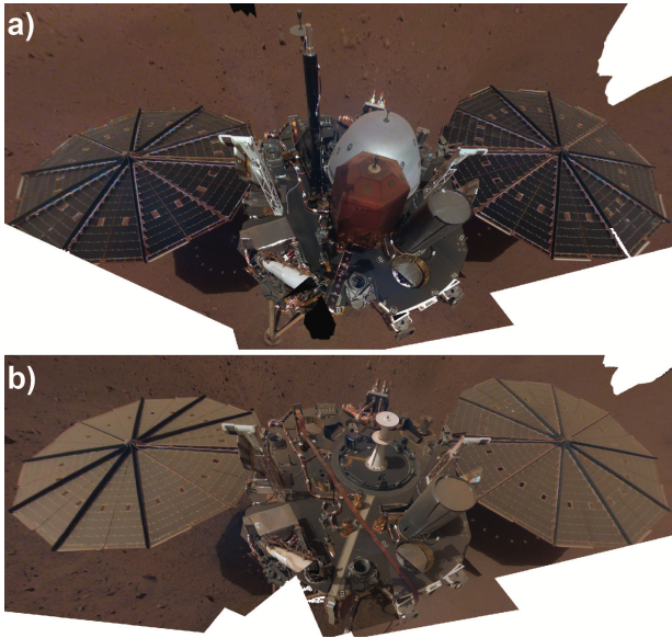
Figure 4. Comparative selfies of the InSight lander reconstituted from images taken by the IDC: a) at the beginning of the mission (Dec. 6, 2018, sol 10), with the instruments (SEIS and HP3) still on the lander; b) after around 100 days (March 15, 2019, sol 106 and April 11, 2019, sol 133), with evidence of dust coating on the lander and solar panels (Image credit JPL/NASA).
