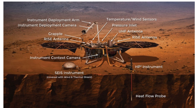
Figure 2. InSight lander artist's concept showing its scientific payload. https://mars.nasa.gov/insight/spacecraft/instruments/summary/
