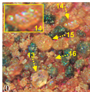
Figure 9. Microscopic observation of sub-rounded to rounded particles of Mars regolith at the Phoenix site. Picture width is 500 \mu\text{m} (Goetz et al. 2010).
