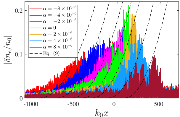
FIG. 7. Snapshots of the EPW amplitude, taken at time \omega_0 t = 4830 , for different chirp rates obtained from 1D PIC simulation. The EPW is driven by two counter-propagating electromagnetic fields (pump and seed) in a plasma profile with a positive density gradient. The black dashed lines represent the curve of Eq. (9).
