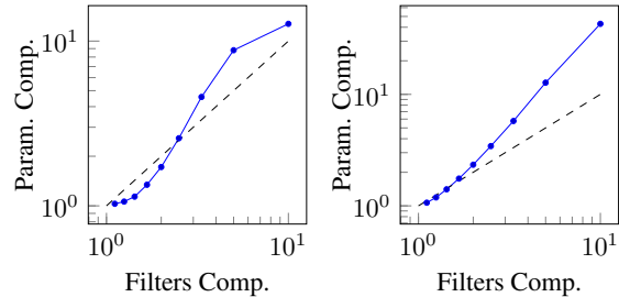
Figure 4. For ResNet-50 on ImageNet (left) or HRNet-48 on Cityscapes (right): relationship between the estimated compression rate in terms of pruned filters (x-axis) and remaining parameters after reducing the network using our method (y-axis). The dashed lines provide a y = x reference.
