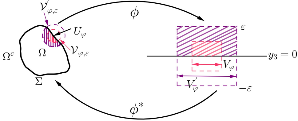
FIGURE 1. Change of coordinates
