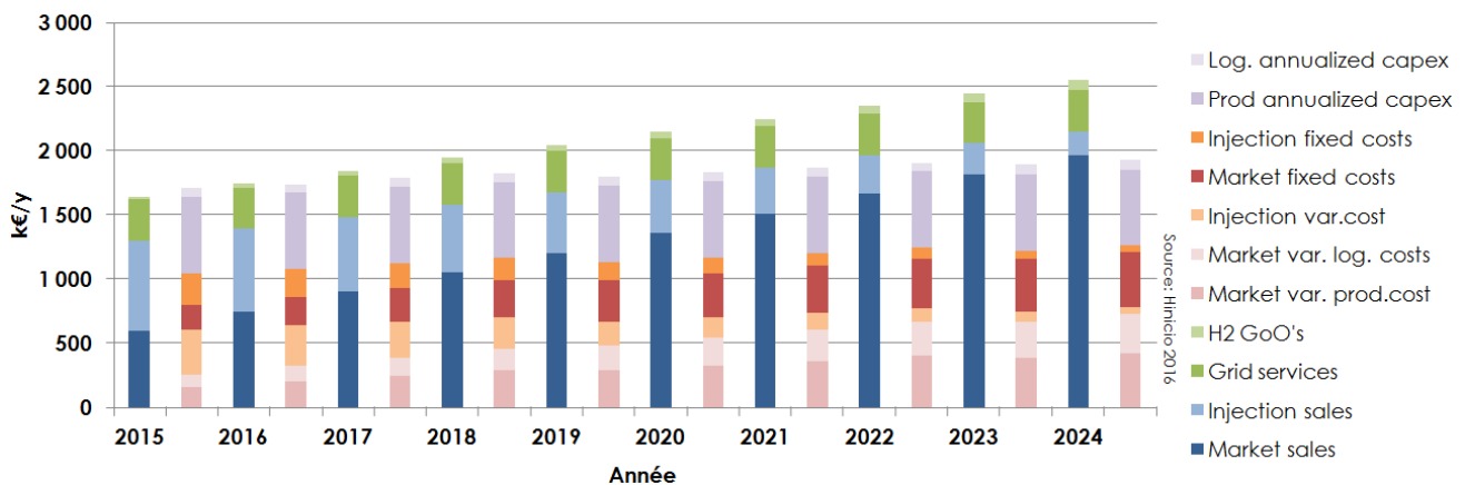
Figure 1. Evolution of annualized revenues (blue and green bars) and costs (purple and red bars) of a 2 MW “semi-centralized water electrolysis "regional" site per [5]. The revenues include sales of the hydrogen on the energy markets and injected in the gas grid, the electricity grid services and “renewable hydrogen” certificates (H2 GoO in the figure). The costs include annualized fixed costs for the logistics and production assets, the fixed and variable costs.
