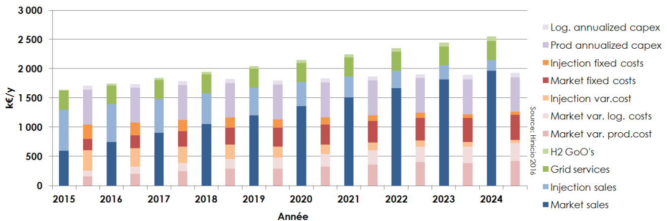
Figure 1. Evolution of annualized revenues (blue and green bars) and costs (purple and red bars) of a 2 MW “semi-centralized water electrolysis” regional site per [5]. The revenues include sales of the hydrogen on the energy markets and injected in the gas grid, the electricity grid services and “renewable hydrogen” certificates (H2 GoO in the figure). The costs include annualized fixed costs for the logistics and production assets, the fixed and variable costs.
