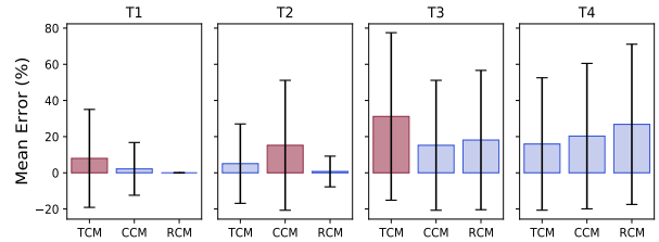
(a) Mean Error Percentage (MEP) per task, per visualization
