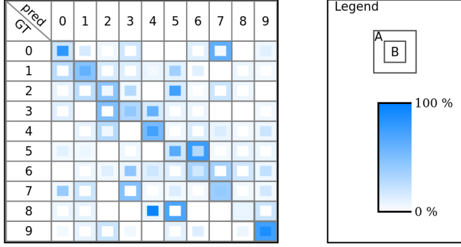
Fig. 2: Example of Combined Confusion Matrix (CCM) representation.
