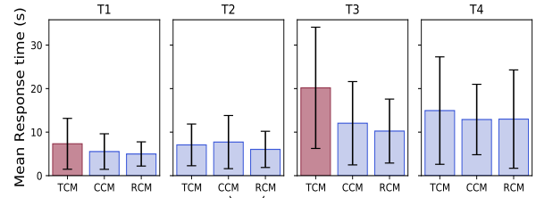
(b) Mean Response time (MRT) per task, per visualization
