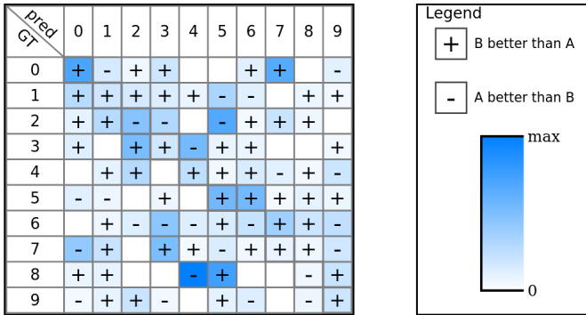
Fig. 3: Example of Relative Confusion Matrix (RCM) representation.
