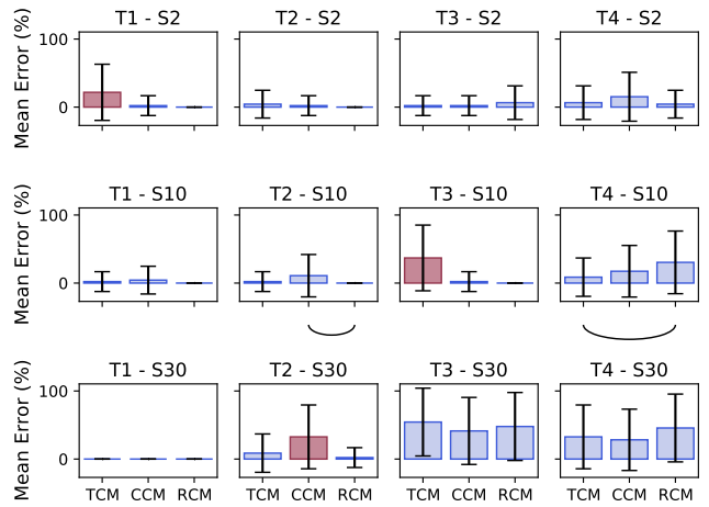
(a) Mean Error Percentage (MEP) per task, per matrix size, per visualization
