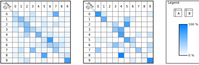
Fig. 1: Example of Twin Confusion Matrix (TCM) representation
