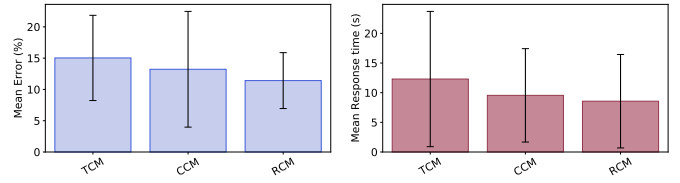
(a) Mean Error Percentage (MEP) per visualization (b) Mean Response time (MRT) per visualization
