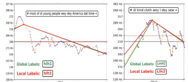
Figure 3: Contours from two categories of topic.
