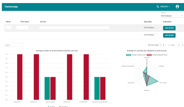
Figure 5: The pedagogical engineers' dashboard
