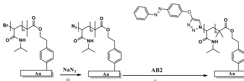
Figure 2. General scheme summarizing the stepwise strategy for the preparation of the multifunctional hybrid plasmonic system (GNPA-PNIPAM-AB). (i) spontaneous covalent grafting of hydroxyl (-OH) terminated aryl diazonium on the surface of the GNPs; (ii) 2-bromoisobutyryl bromide (0.1 M, toluene), trimethylamine (0.12 M), 5 min. (iii) NIPAM in Surface-Initiated Atom Transfer Radical Polymerization (SI-ATRP) conditions. (iv) \text{NaN}_3 (0.05 M, DMF) for 24 h, rt (v) \beta -cyclodextrin (1.25 mM), AB2 (0.05 M), Cu(II) sulfate pentahydrate (2.5 mM), L-ascorbic acid sodium salt (7.5 mM) in water under Ar at room temperature, 24 h.
