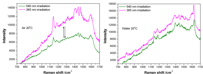
Figure 9. SERS spectra excited at 633 nm, of a selected GNPA-PNIPAM-AB sample (array D140), upon repetitive cycling irradiations to UV (365nm, pink line) and visible (540nm, green line) light, each of 1h duration. Spectra were recorded in air (left) and in water (right), at room temperature (20°C).
