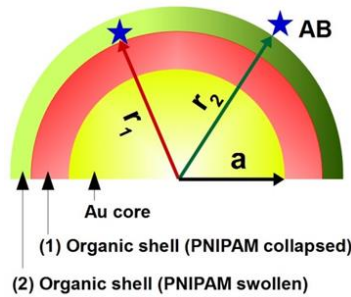
Figure 7. Schematic representation of a hemi-sphere GNP surrounded by an organic shell with a AB photochromic unit. Where a is the radius of the hemi-spheric NP; r_1 and r_2 the distance from the AB unit to the GNP center, in the collapsed (1) and swollen (2) state of PNIPAM.
