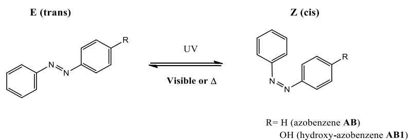
Scheme 2. Reversible isomerization of azobenzene moieties upon UV-Vis irradiation. The trans ( E ) isomer is planar and the cis ( Z ) isomer is bent and more compact.
