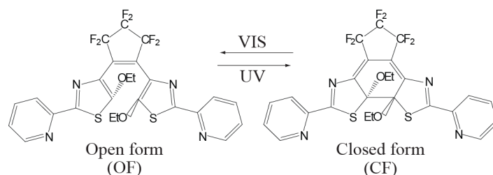
Scheme 1. Reversible photoisomerization in diarylethenes family upon UV-Vis light irradiation.
