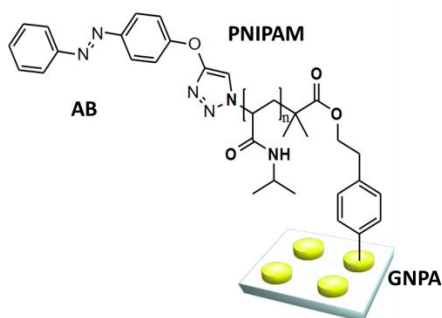
Scheme 3. Illustration of the attachment of an azobenzene derivative on PNIPAM brushes grafted on GNP Arrays.
