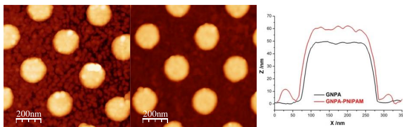
Figure 3. AFM images and height profiles in air at room temperature of GNPA (left and black curve) and GNPA-PNIPAM (right and red curve).
