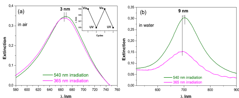
Figure 5. (a) Extinction spectra of a GNPA-PNIPAM-AB sample (array D140) upon repetitive cycling irradiations to UV (365nm, pink line) and visible (540nm, green line) each of 90 min duration. (a) Recorded in air at room temperature (20°C); the reproducible cycles are shown in the inset. (b) Recorded in water at room temperature (20°C); poor reproducibility of the cycles in this case (not shown). Either in air or in water, exposure to UV light led to cis isomer with a blue shift of the LSPR band while 540 nm green light led to trans isomer with a red shift of similar amount.
