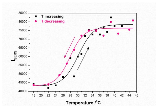
Figure 8. Integrated SERS intensity, of the 1142 \text{cm}^{-1} Raman line of AB, versus temperature for one selected GNPA-PNIPAM-AB sample (D 140).
