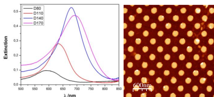
Figure 1. (a) Extinction spectra of four GNPs (disk diameter D= 80, 110, 140 and 170 nm) recorded in air at room temperature. These spectra were recorded with a spectrometer (LOT ORIEL, 74050 model, 400-1000 nm spectral range) equipped with a CCD camera (ANDOR, CCD-8855) under an upright optical microscope (Olympus, BX51TF) through a 100 x objective (Olympus, NA: 0.8) (b) AFM image of one array (D140) obtained in air at room temperature
