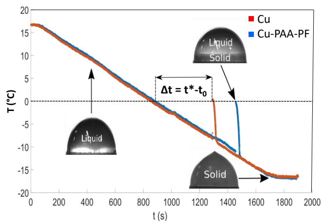
Figure 5. Temperature of sessile droplets ( 100\ \mu\text{L} ) monitored by IR camera as a function of time (after 10 cycles). The drop profiles, recorded by the CCD camera, are added as a guide.
