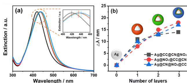
Figure 3. (a) Normalized UV-vis spectra of Ag NPs (black line), Ag@CN (red line), Ag@CN@NO 2 (green line) and Ag@CN@NO 2 @CCH (blue line); (b) Plot of \Delta\lambda (red shift of plasmon band) vs the number of grafted layers around Ag cores for the step-by-step functionalization of Ag@CCH@CN@NO 2 , Ag@NO 2 @CCH@CN and Ag@CN@NO 2 @CCH.
