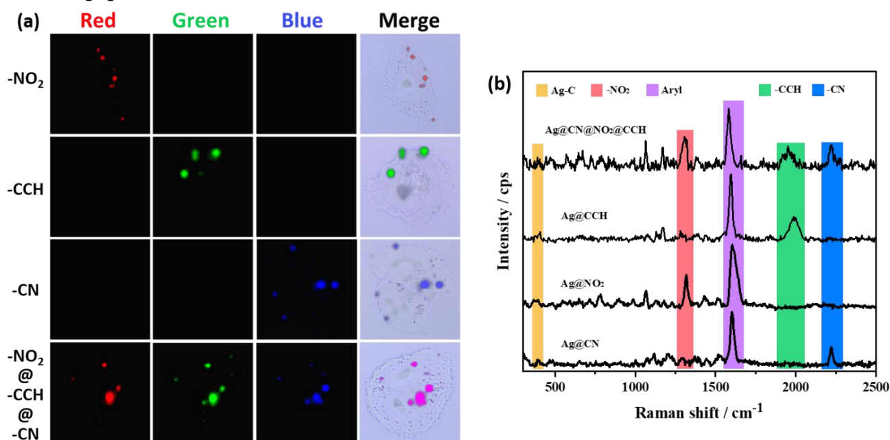
Figure 6. (a) Raman images of HELA-HSP70/GFP cells after uptake of various SERS labels (re-suspended with 2 mL of medium to reach 20 \mu\text{g}\cdot\text{mL}^{-1} ), as indicated on the left panel: Ag@NO 2 , Ag@CCH, Ag@CN and Ag@CN@NO 2 @CCH. The right column displays the overlay images of cell bright field pictures and Raman images. Scale bar: 5 \mu\text{m} . The Raman spectra in the red, green, and blue channels correspond to the signals of NO 2 , CCH and CN, respectively. (b) Corresponding SERS spectra for each SERS tags. The SERS images were obtained with a 638 nm laser (30 mW) and a 100 \times objective lens.
