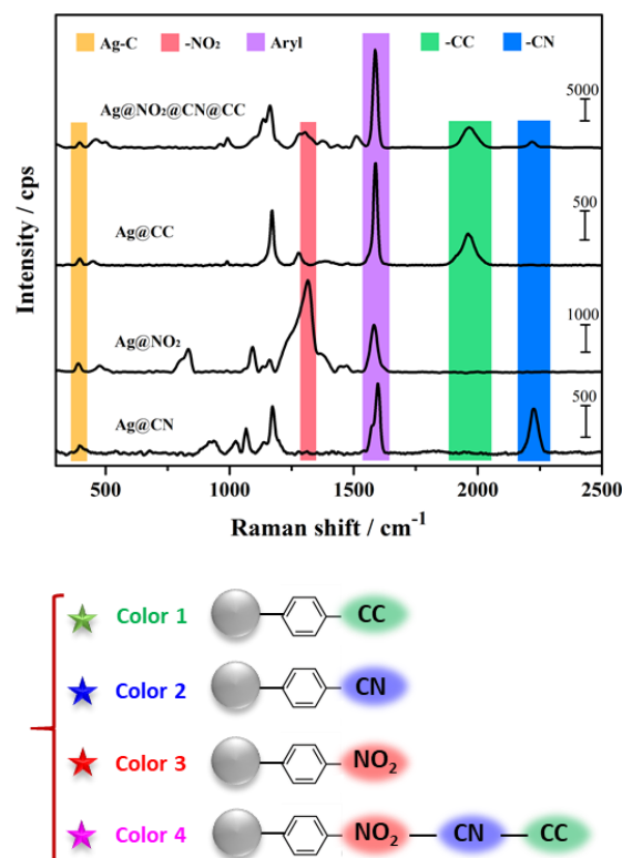
Figure 5. SERS spectra of the three single layer-SERS tags and multilayer-coated Ag@NO 2 @CN@CCH NPs. The excitation wavelength was 638 nm, and the exposure time was 2 s. The molecular structures of the three Raman reporters derived from aryl diazonium salts and the multilayer-coated Ag@NO 2 @CN@CCH NPs are illustrated below.
