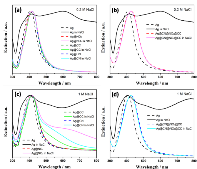
Figure 4. Normalized UV-vis spectra of bare Ag NPs coated by (a, c) single polyaryl layers or (b, d) multilayers, before (dotted lines) and after (full line) addition of (a, b) NaCl (0.2 M) or (c, d) NaCl (1M). It is noteworthy that 0.01 wt% PVP was present in all functionalized Ag NPs samples.
