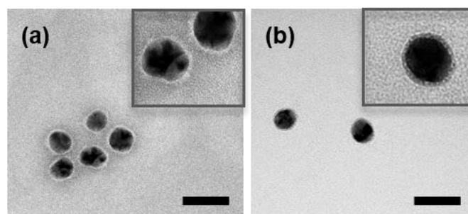
Figure 2. Typical TEM images of (a) bare Ag NPs and (b) Ag@NO 2 . Scale bar = 50 nm. The insets show zoom of each figure to better observe the surface coating.
