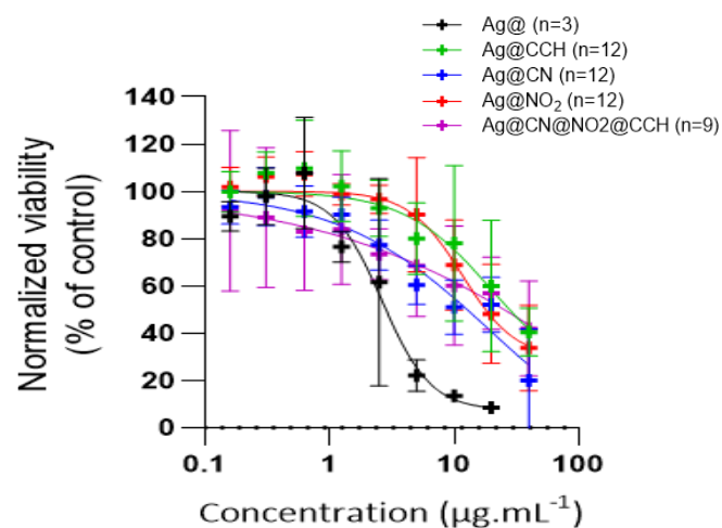
Figure 7. Viability of HELA-HSP70/GFP cells after incubation with different amounts of SERS labels and bare uncoated Ag NPs, for 6 hours.
