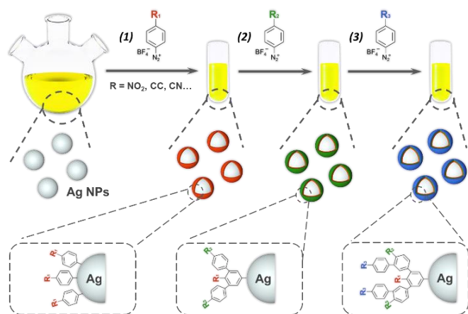
Figure 1. Representative scheme of the preparation process of SERS encoded tags based on aryl diazonium salt chemistry. Aqueous Ag NPs solutions were mixed with aryl diazonium salts bearing different Raman reporter groups ( R_{1-3} = \text{NO}_2, \text{C}\equiv\text{CH}, \text{C}\equiv\text{N} ), following a sequential process.
