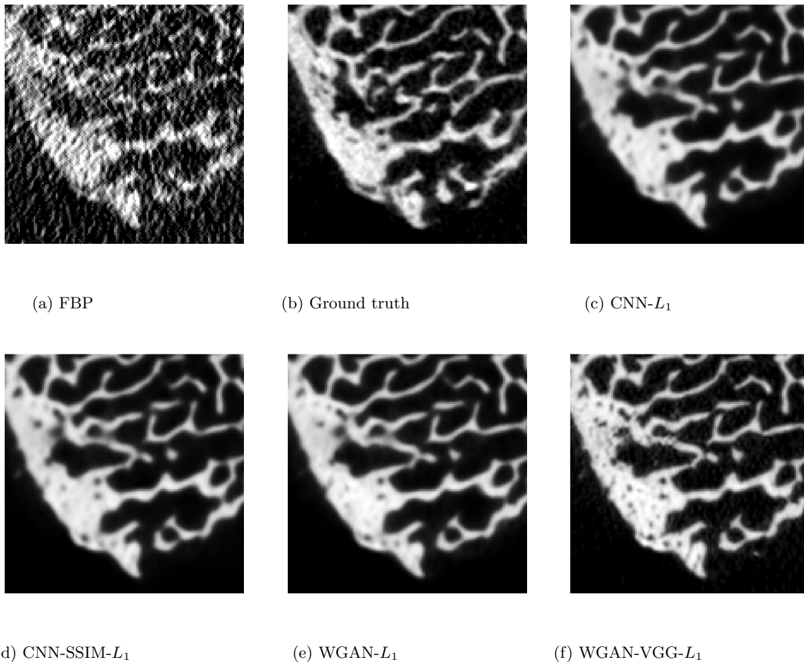
Figure 4: ROI from volume 1 of size 140 \times 140 voxels obtained with different methods. Window size is [-1000, 3000] HU. FBP is obtained after simulation of 10% of the normal dose to obtain the projections from the ground truth. Networks are fed with this FBP as input.
