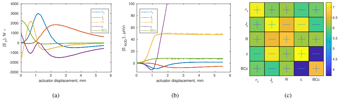
Figure 20: Sensitivities in force ( S_F ) (a) and NOD ( S_{NOD} ) (b). (c) Absolute Hessian matrix [H] expressed in decimal logarithm for sample MZ5-S1450G.
