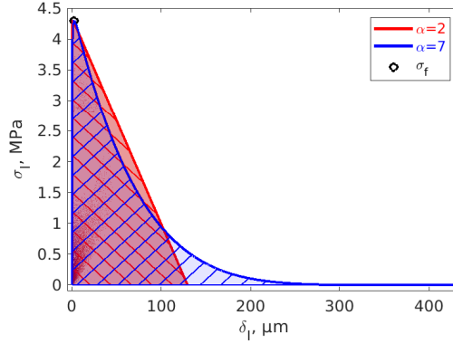
Figure 5: Mode I traction-separation law using the initial parameters of the PPR model (Table 1). The cohesive strength \sigma_f corresponds to the maximum traction (black circle), and the fracture energy J_c is the integral of the traction-separation curve (dashed areas).
