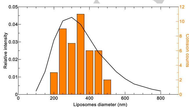
Figure 3. Size distributions from DLS data (black line) and from charge data by integrating current spikes of i-t curve recorded at +0.7 V vs Ag/AgCl on 10 \mu\text{m} Pt UME in 500 nM RL 0.1 M PB at pH 7.4 at 15 min after addition of 3 \mu\text{M} redox DMPC liposomes (orange bar).
