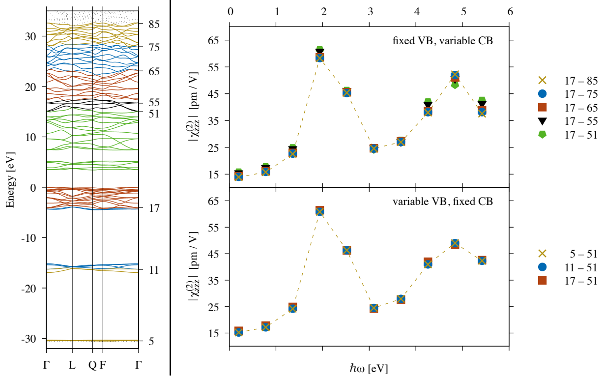
FIG. 11. Lhs: Band structure of LiNbO 3 , in which the energy relative to the valence band maximum is given on the left axis and the corresponding band indices (cf. rhs) are given on the right axis. Rhs: Resulting SHG spectra of LiNbO 3 calculated with different Kohn-Sham basis sets. In the bottom (top) half of the figure, the lower (higher) boundary of the band range of the Kohn-Sham basis is varied, while the higher (lower) boundary is fixed. In each case, the corresponding band indices are given in the key. These calculations are all performed with a 4 \times 4 \times 4 grid of k -points. VB and CB stay for valence and conduction bands, respectively.
