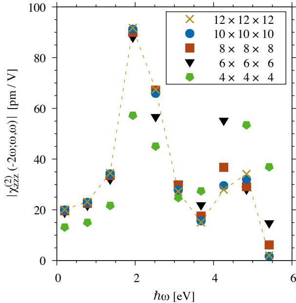
FIG. 12. Resulting SHG spectra of LiNbO 3 calculated with different number of subdivisions regarding the discretization of the Brillouin zone. All calculations are performed with a Kohn-Sham basis consisting of bands 11 – 75.
