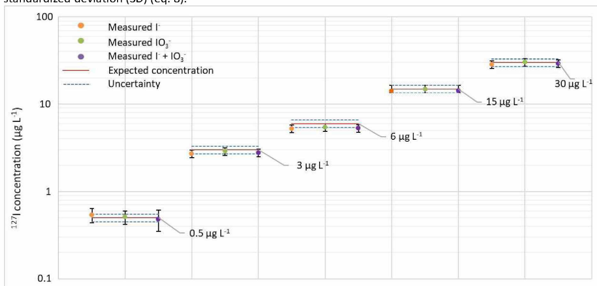
Figure 10 - ^{127}\text{I} quantification in synthetic samples in mass-shift mode in OM. Error bars represents calculated uncertainties
