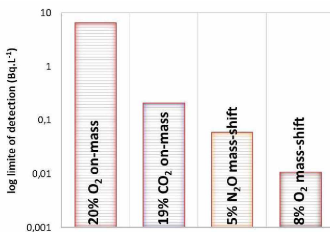
Fig. 8 - Obtained limits of detection with different gas and modes with a microFlow inert PFA nebulizer in OM.
