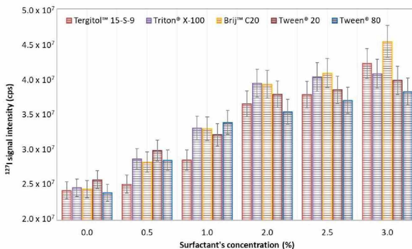
Fig. 2 - ^{127}\text{I} 100 \mu\text{g L}^{-1} ICP-MS signal intensity (cps) in 0.1% (v/v) NH_4OH using different surfactants: Tergitol™ 15-S-9, Triton® X-100, Brij™ C20, Tween® 20 and Tween® 80. On-mass measurement mode. Error bars represent 10%.
