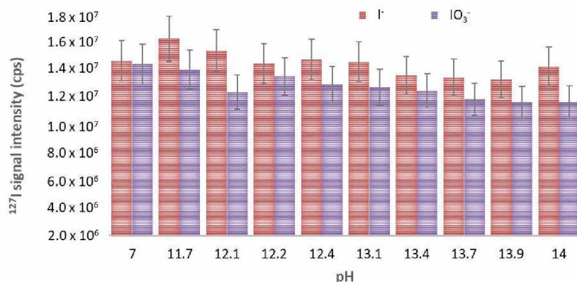
Fig. 1 ICP-MS signal intensity (cps) variation for 100 \mu\text{g L}^{-1} of ^{127}\text{I} in NH_4OH solutions ranging from pH 7 to 14. On-mass measurement mode. Error bars are estimated at 10%.
