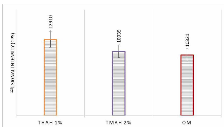
Figure 5 - Signal intensity at m/z 129 for Blanks of 3 media. On-mass measurement mode. Error bar represents 10%.
