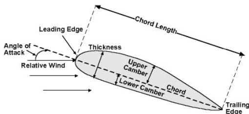
Figure 6: Technical vocabulary of a NACA profile.
