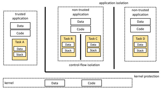
Figure 2: Isolation Boundaries in AUTOSAR [35]
