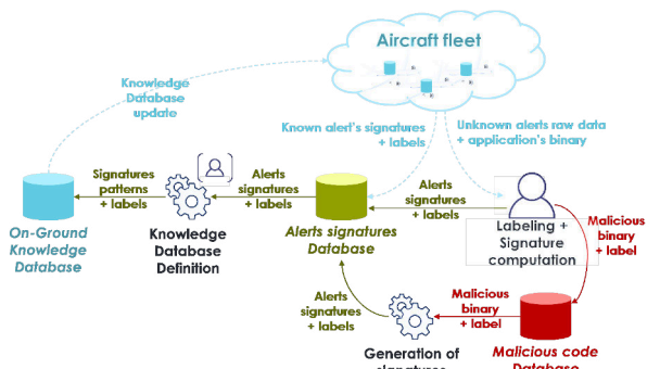
Fig. 5. Knowledge database of anomalous behaviour, as defined in [21]
