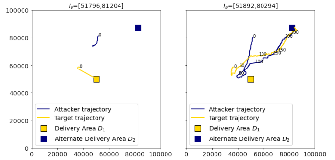
Fig. 9: Analysis of trajectories in S2 scenario for v_a^{max}
