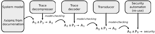
Fig. 2. Proof strategy
