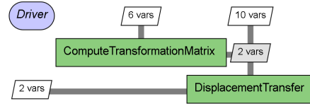
Figure 8: DispTransferGroup XDSM.
