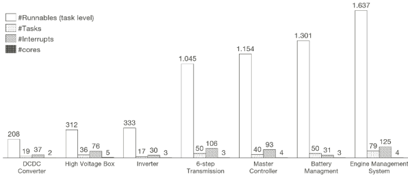
Fig. 1. Number of cores, tasks and runnables of different automotive applications
