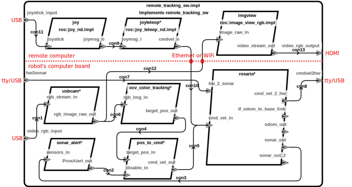
Fig. 1. Robotic application.
