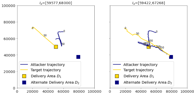
Fig. 8: Analyse of trajectories in S3 scenario for v_a^{max}
