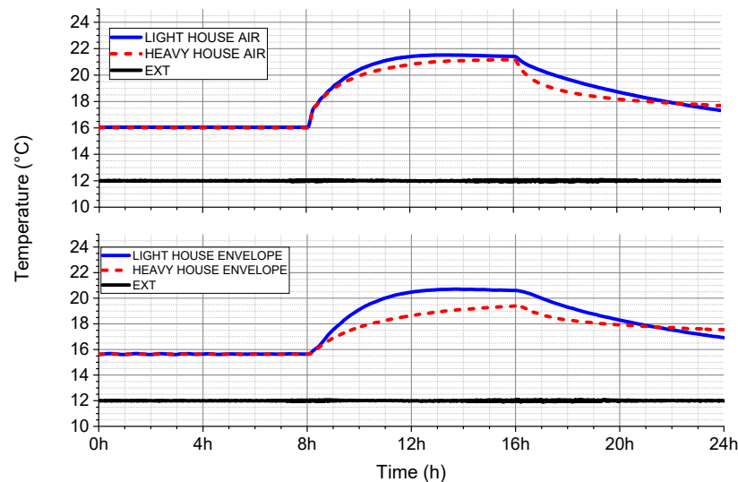
Figure 20. Experimental temperature evolution in the test chamber (upper: mean air temperature, bottom: mean envelope temperature).
