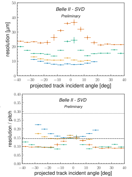
Figure 3: Cluster position resolutions (top) and resolutions normalised to the sensor (bottom) as a function of the incident angle of the track traversing the sensor are shown. Results are obtained on 98 \text{ pb}^{-1} collision data from 2020 run.
