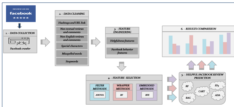
Fig. 2: The workflow adopted in this study
