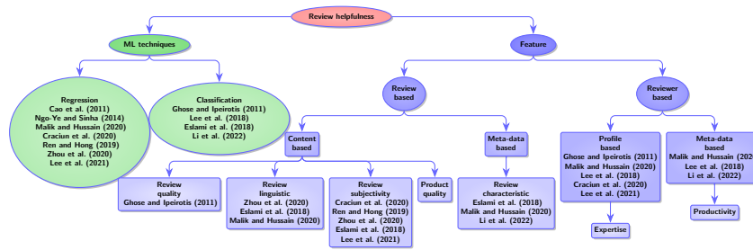
Fig. 1: Helpful review prediction studies in the literature
