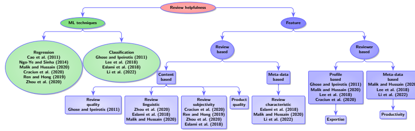
Fig. 1: Helpful review prediction studies in the literature
