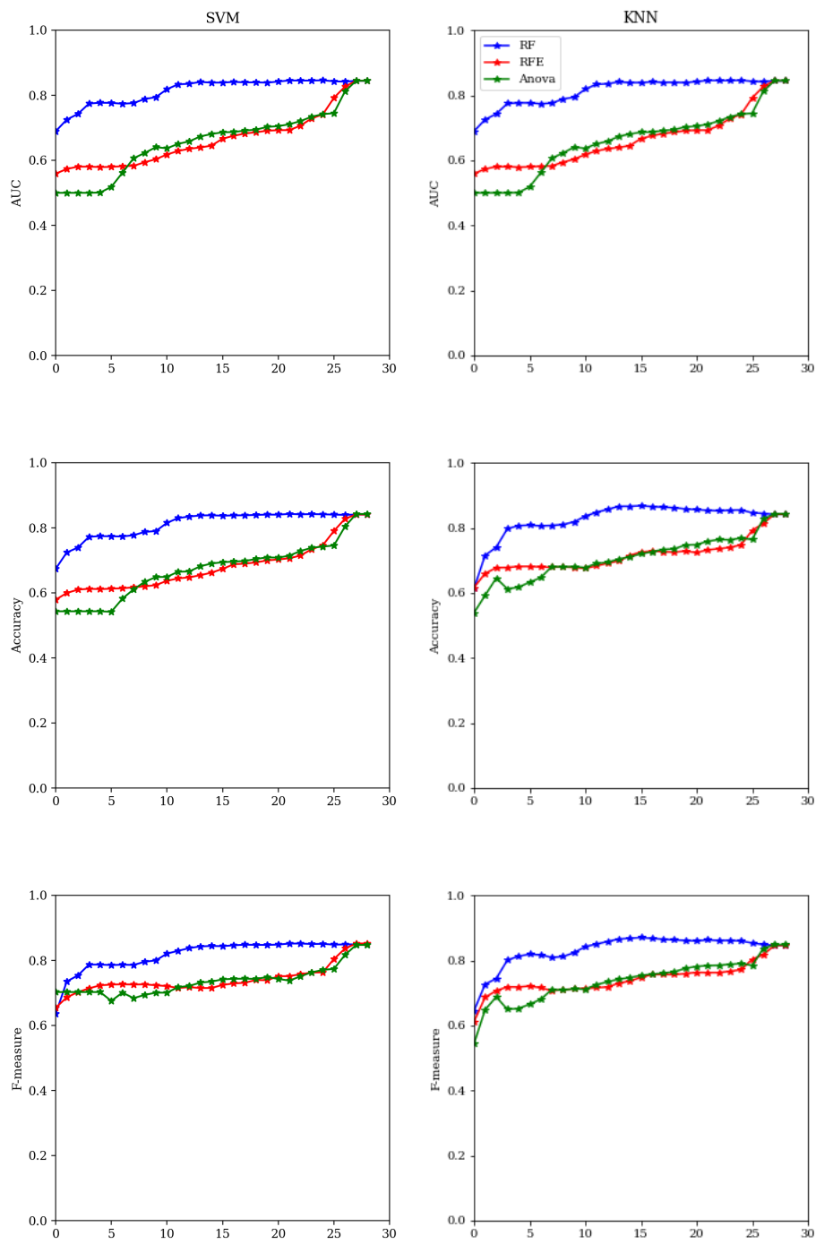
Fig. 6: Feature selection methods' performance
