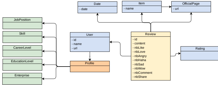
Fig. 3: Structure of the collected data
