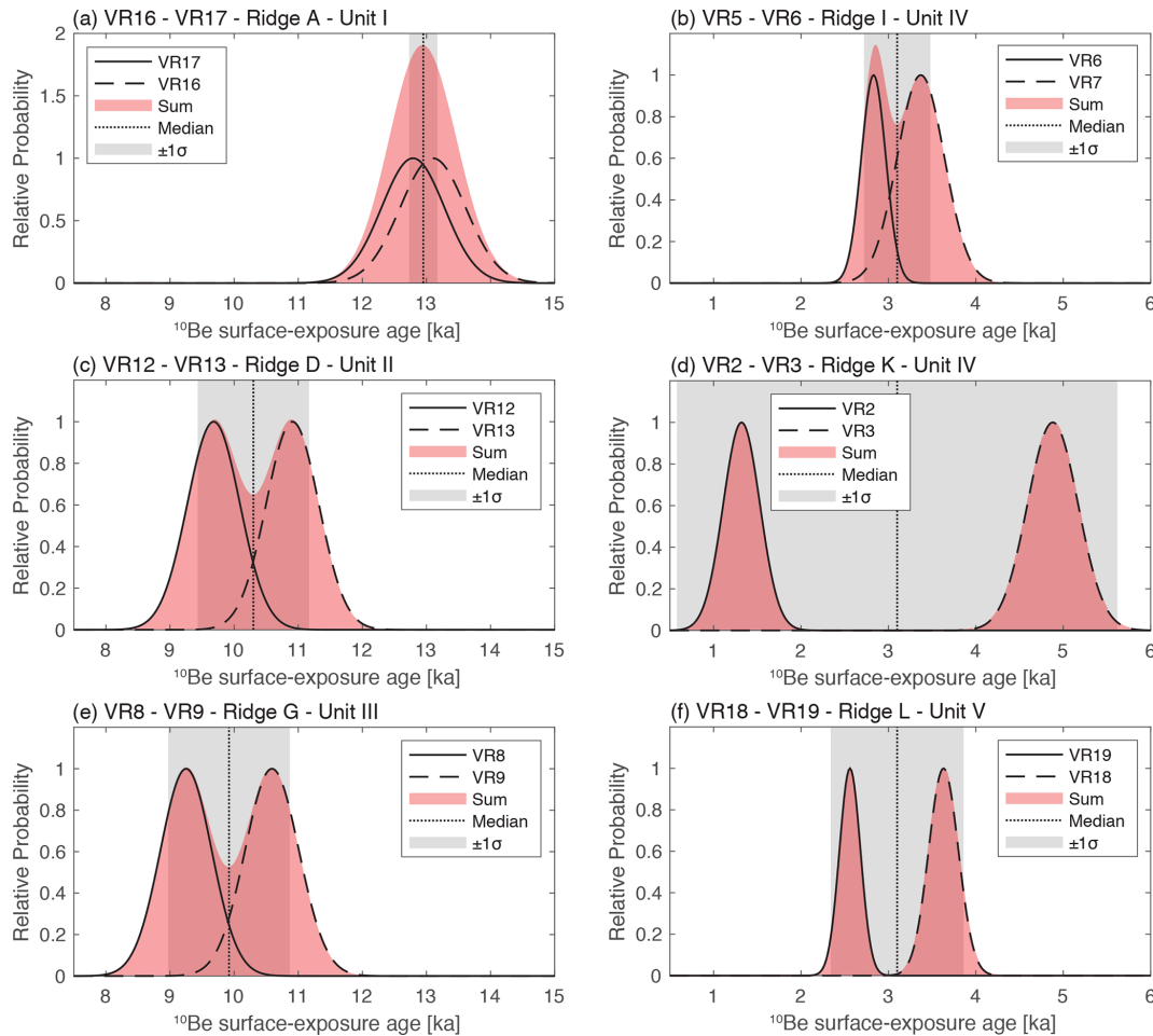
Figure 8. Probability distributions of the individual 10 Be surface-exposure age, sum, and median for each ridge (similar results are shown in Fig. A4 for each unit).
