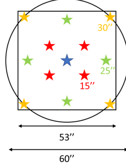
Figure 5: Directions used for the jitter/SR computation in the FoV of diameter 60". The square of side 53" corresponds to the large MICADO FoV. The stars are distributed as follows: 1 star on axis, 4 stars at 15", 4 stars at 25" and 4 stars at 30". When the small MICADO FoV is considered (20×20"), we average from 1 star on axis and 4 stars at 10" (placed in the same manner as the 4 stars at 15").
