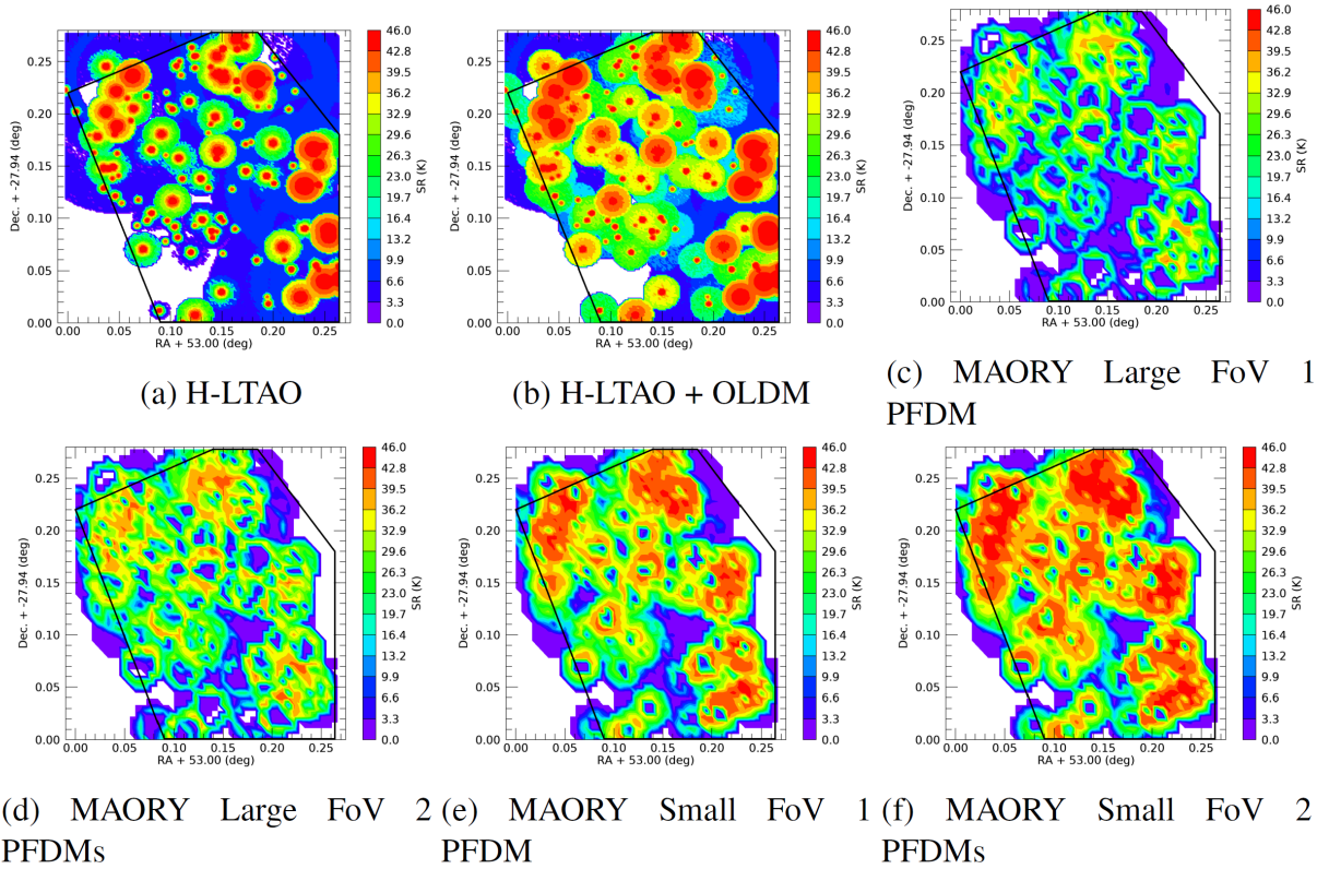
Figure 19: Strehl ratio in K band with H-LTAO (on axis) or with MAORY (averaged on the scientific FoV) for the GOODS-S field. The black lines indicate the area used for the sky coverage computation.
