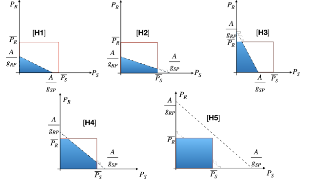
Fig. 2. Feasible set of (OCF).
