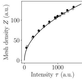
Figure 8: The mesh density Z as a function of the intensity of the point-process \tau (line: \mu_{\text{St}}(\tau; Z) in equation (22) , unitary area). Gmsh results with “MeshAdapt” strategy (points) and with “Frontal” strategy (open circles); Cast3m result (cross); Triangle result (filled square); Abaqus result (open square). Corresponding meshes are given in figure 6 and figure 7 .
