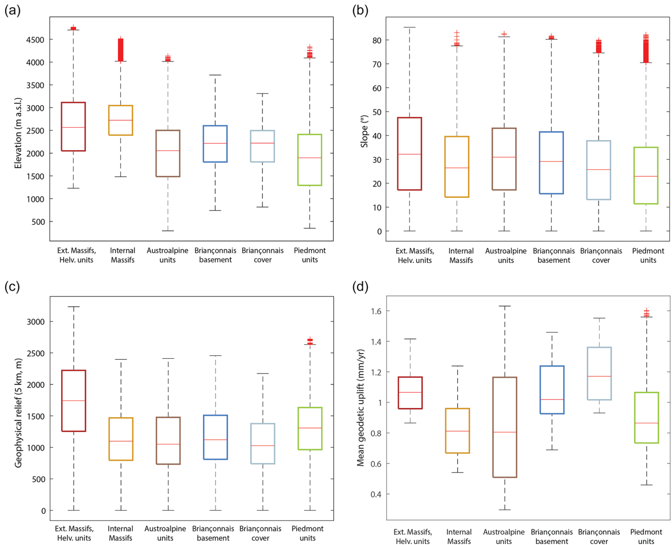
Figure 7. Box-and-whisker plots for the spatial distribution of elevation (a) , slope (b) , 5 km geophysical relief (c) and mean geodetic uplift (d) within the entire DB catchment, classified by individual lithotectonic unit. The horizontal red line represents the median of each distribution; bottom and top of each box are the 25th and 75th percentiles. Whiskers extend up to 1.5 times the interquartile range; outliers (red crosses) are observations beyond the whiskers.
