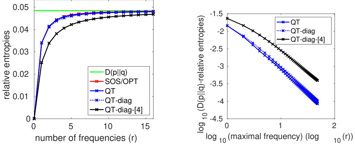
Figure 1: Comparison of relative entropy estimates for several numbers of frequencies, showing the effect of varying r . Left: D(p||q) is the exact value, with moment-based approximations OPT/SOS (here equal), and the ones based on quantum information divergences, with full metric learning (QT) or diagonal metric learning (QT-diag), with also the use of the weaker quantum divergences proposed by [4]. In several cases the red curve associated with OPT/SOS bounds is not visible as it coincides with the blue curve of QT bounds. Right: same experiment without OPT/SOS, with deviation to f -divergence reported in a log-log plot.
