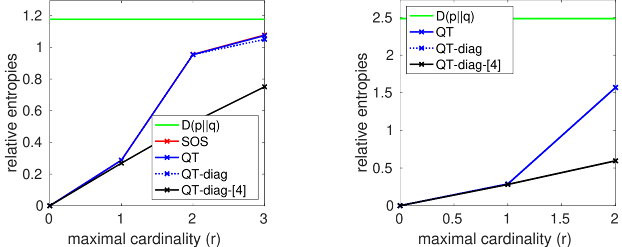
Figure 3: Comparison of relative entropy estimates for several numbers of frequencies for all subsets of cardinality less than r , for n = 10 and n = 20 . D(p||q) is the exact value, with moment SOS-based approximations, and the ones based on quantum information divergences, with full metric learning (QT) or diagonal metric learning (QT-diag), with also the use of the weaker quantum divergences done by [4].
