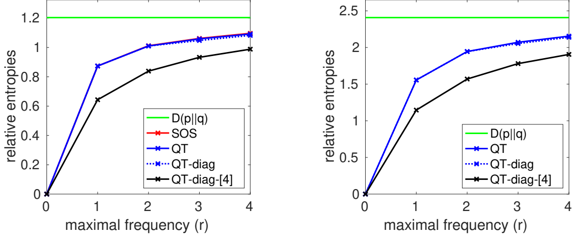
Figure 2: Comparison of relative entropy estimates for several numbers of maximal marginal frequency r , for n = 2 (left) and n = 3 (right). D(p||q) is the exact value, with moment SOS-based approximations (only plotted in the left plot, and for which we only compute the cost function of Eq. (18) with the optimal quantum solution from Eq. (20), which is close to optimal for Eq. (18)), and the ones based on quantum information divergences, with full metric learning (QT) or diagonal metric learning (QT-diag), with also the use of the weaker quantum divergences done by [4].
