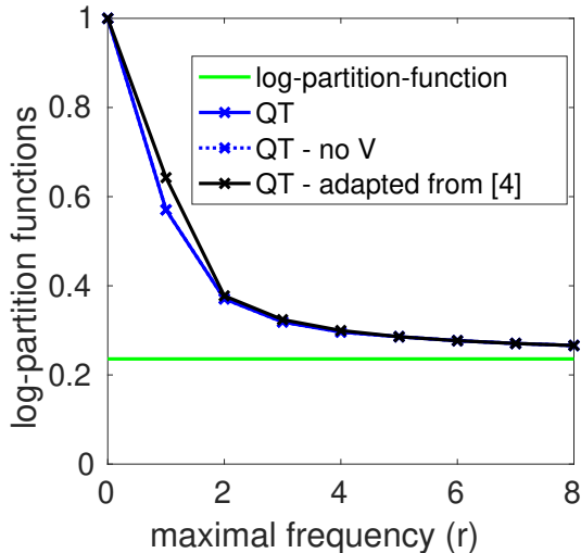
Figure 4: Comparison of log-partition function estimates for several numbers of frequencies for n = 1 . See text for details.
