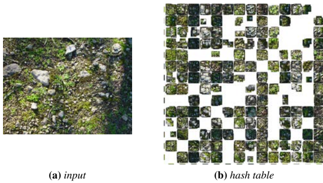
Figure 11: Description of regions' content. All tiles of an input are given keys (k_1, k_2) (row, column) stored in a hash table. The keys are obtained from our label-maps. The hash table allows tiles to be instantly selected according to their content.
