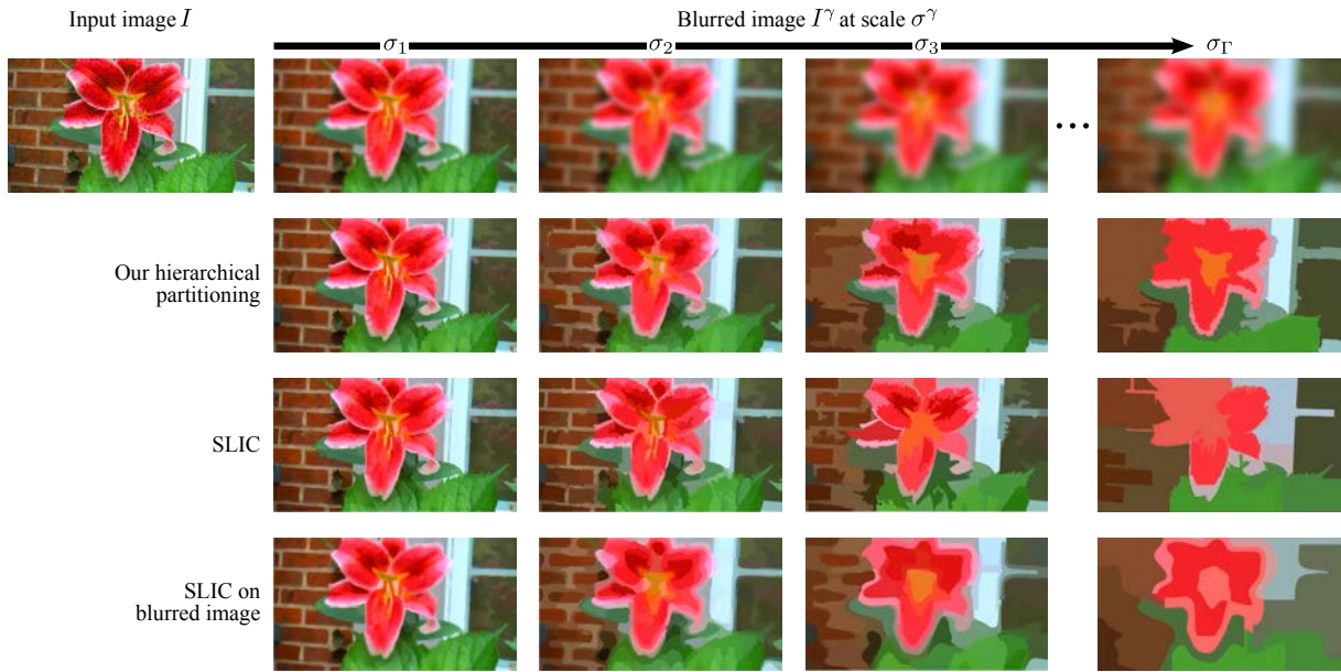
Figure 2: Superpixel decomposition from our hierarchical algorithm (2nd row) compared to the SLIC algorithm on the original (3rd row) and on a blurred image (4th row). The average color of each superpixel is represented here.
