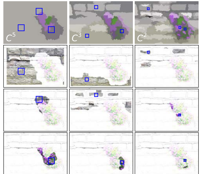
Figure 10: Content similarity. For each level l of the label-map (3 levels, top row) we show three patches R outlined in blue. \rho_l decreases from left to right, and the size of the patches decreases accordingly. Rows two to four highlight subsets of pixels that are centers of patches of the same size, so that the histogram is “similar” to h_R^l (in this case, we consider histograms as similar if their two most frequent labels are matching).
