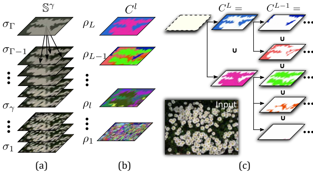
Figure 5: Multi-scale labeling. Based on the dense hierarchy of superpixels (a), a few representative levels are selected to build a multi-scale label-map (b). It can be seen as a tree of clusters (c).
