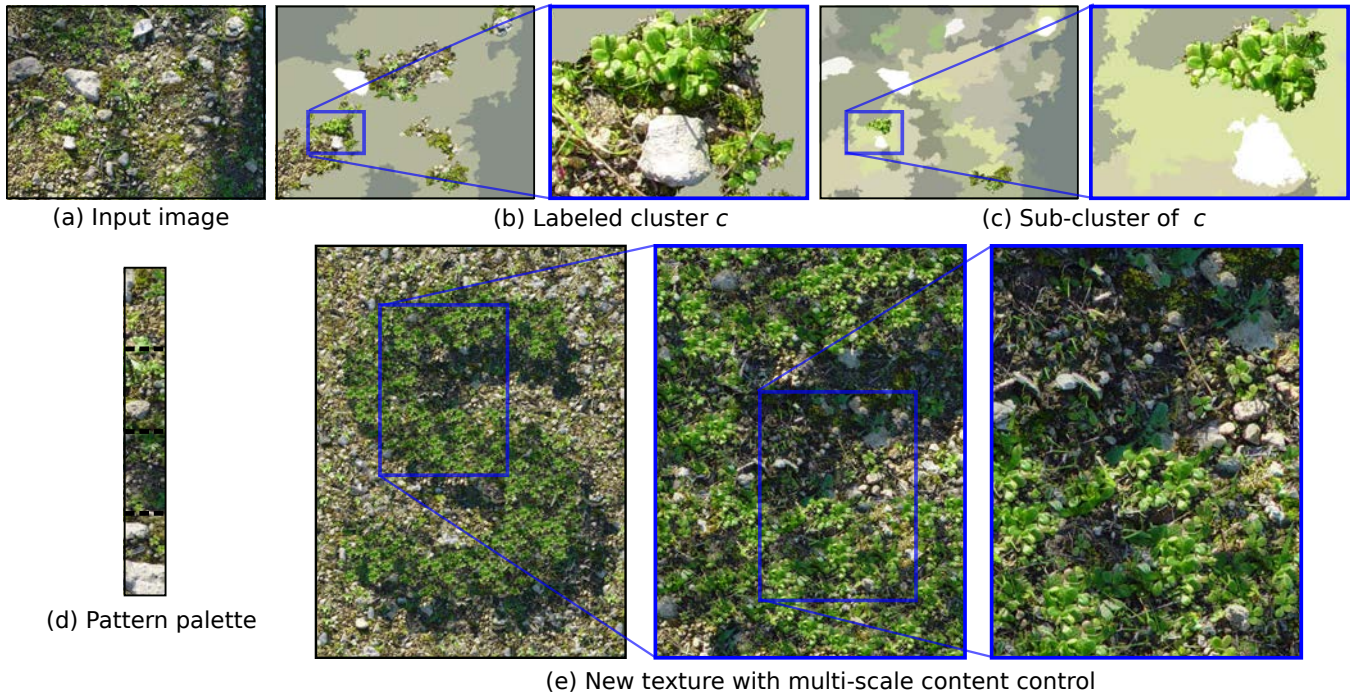
Figure 1: The input image (a) is a non-stationary texture. Our multi-scale analysis provides a hierarchy of labeled clusters: one cluster at a coarse scale (b) includes sub-clusters at finer scales (c). It has several applications in texture synthesis, such as automatic pattern palettes for interactive texture editing (d) and content selection for creating new non-stationary textures (e).
