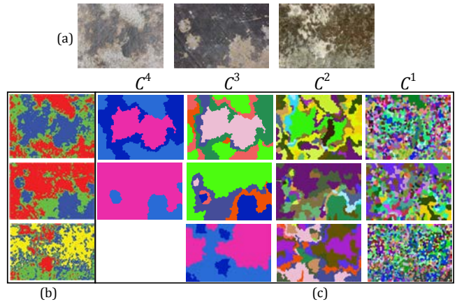
Figure 7: Comparison of our label-maps to the labeling results of Layered-Shape Synthesis [Rosenberger et al. 2009]. (a): Input images (from left to right); (b): corresponding Layered-Shape Synthesis label-maps (top to bottom); (c): Our label-maps (4 levels for the two leftmost input images, and 3 levels for the rightmost one).
