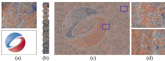
Figure 12: Non-stationary texture synthesis is guided by region description. An example ( 2560 \times 1920 ) and a guidance map are given as input (a). Our label-map is used to describe tiles by keys (b) which are linked to the guidance map. The result of quilting ( 16638 \times 11776 ) is shown (c) with close-ups (d).
