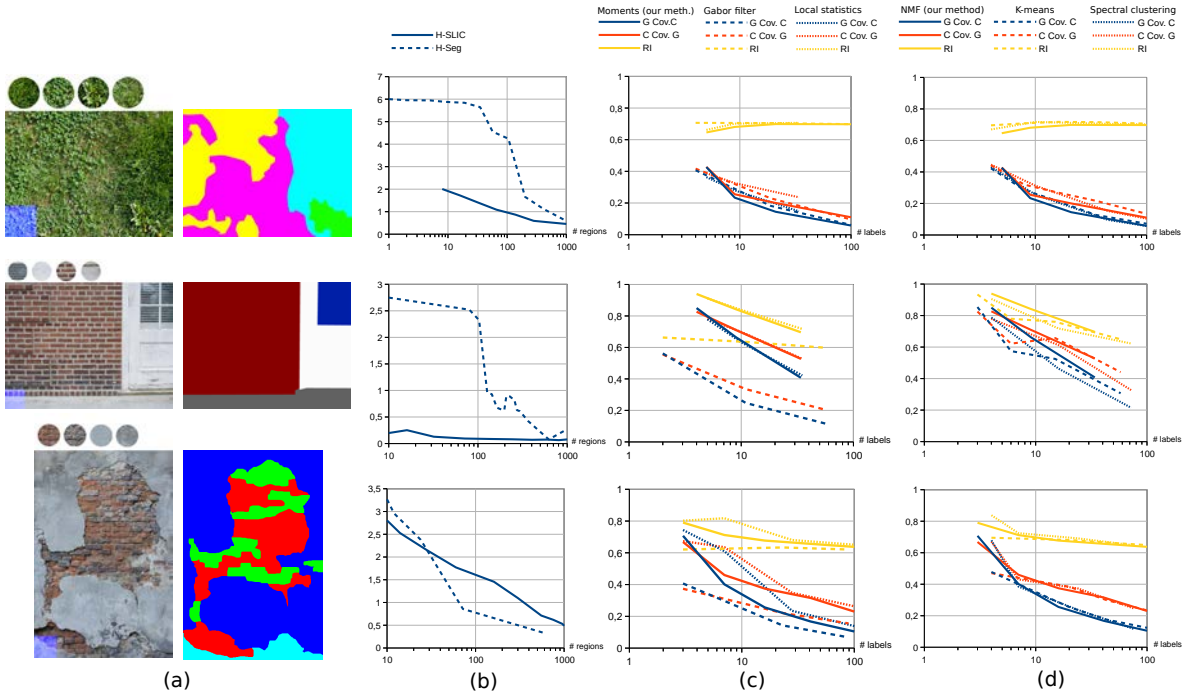
Figure 3: Evaluation. (a) Input images with manual texture labeling taken as ground truth. (b) Our H-SLIC partitioning is compared to hierarchical segmentation using under-segmentation error (the lower the better). Our labeling is tested with alternative feature vectors (c) and compared to other clustering methods (d) using Rand index and covering measures (the higher the better).
