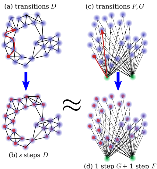
Figure 4: Random walks on a bipartite graph. Each superpixel is represented by a 15D feature point which is a node of the directed k -nearest-neighbor graph (a) with transition probabilities based on the similarity between pairs of SPs. For any given starting node, random walks with several steps provide a similarity map represented by intensity of red dots in (b). Our algorithm approximates the similarity maps by a bipartite graph (c) with a small set of new ‘‘cluster-nodes’’ (green). The walker jumps only twice: from a SP-node to a cluster-node, and back to a SP-node. The goal is to construct such a graph that’s destination probability (d) approximates the similarity maps (b).
