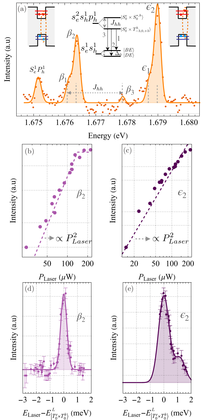
FIG. 6. (a) PL spectra of the p_e - s_h and s_e - p_h transitions from the biexcitonlike complexes s_e^1 s_h^2 p_e^1 and s_e^2 s_h^1 p_h^1 , when the laser is tuned to the energy of the (s_e^1 s_h^1 p_e^1 p_h^1)_{\text{triplet}} TPE condition. The inset represents the levels diagram and the emission paths for s_e^2 s_h^1 p_h^1 . The s -shell recombination of |T_{\pm 1}^e \times T_{\mp 3}^h\rangle allows to detect the signal from s_e^1 p_h^1 indicated by the line at 1.6752 eV. (b), (c) PL intensity of \beta_2 and \epsilon_2 as a function of the laser power. (d), (e) PLE intensity of \beta_2 and \epsilon_2 as a function of the ps -laser energy. The resonant line of \epsilon_2 is incomplete on the low-energy side due to the increase of the laser scattering.
