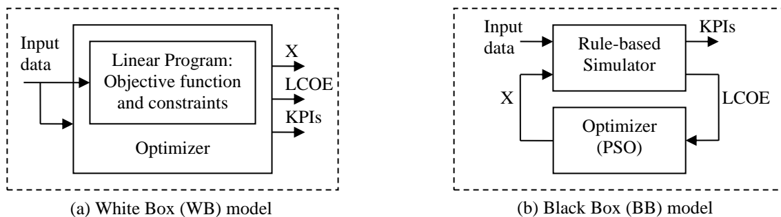
Figure 1. Diagrams of White Box (a) and Black Box (b) models for microgrid design optimization.
