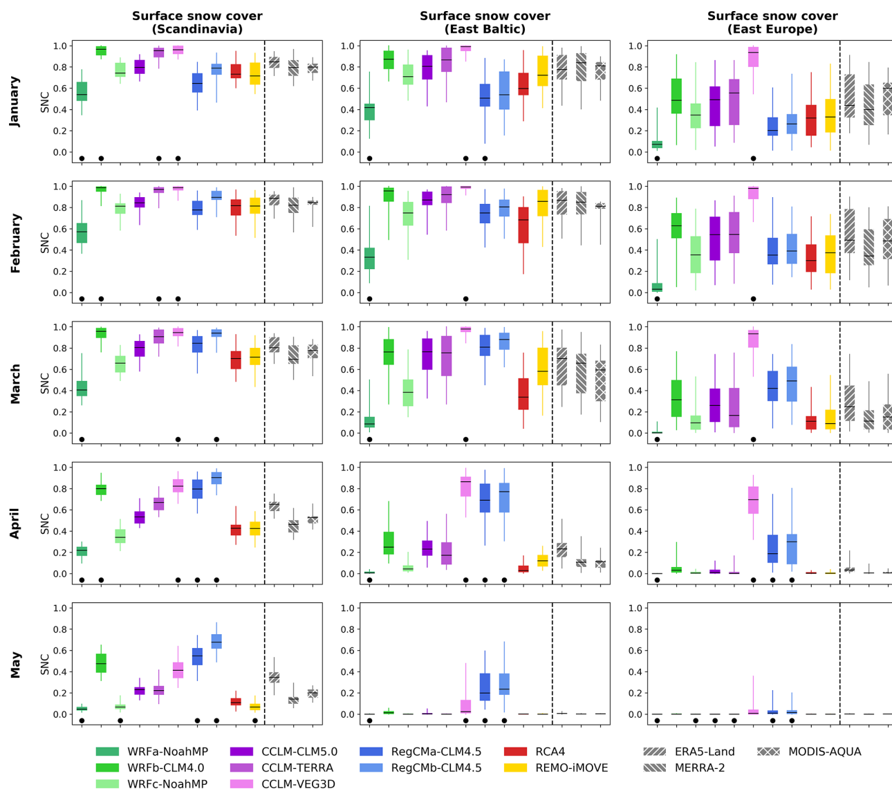
Figure 5. Snow cover for the 10 RCMs, the reanalyses of ERA5-Land and MERRA-2, and the satellite observations of MODIS-AQUA for January to May. The box-and-whisker plots show the interannual variability in snow cover over 1986–2015 for models and reanalyses and over 2003–2015 for satellite observations. Bars represent the median, boxes the interquartile range and whiskers the minimum/maximum values. Dots indicate models lying outside the range of the reference datasets of MERRA-2, ERA5-Land and MODIS-AQUA, i.e., the 25th (75th) model percentile is higher (lower) than the highest 75th (lowest 25th) quantile of the reference datasets. For satellite observations we only use data from days and pixels with less than 50 % cloud cover. See Fig. S1 in the Supplement for the same figure including data for MODIS displayed for cloud cover fraction thresholds of 50 % and 20 %.
