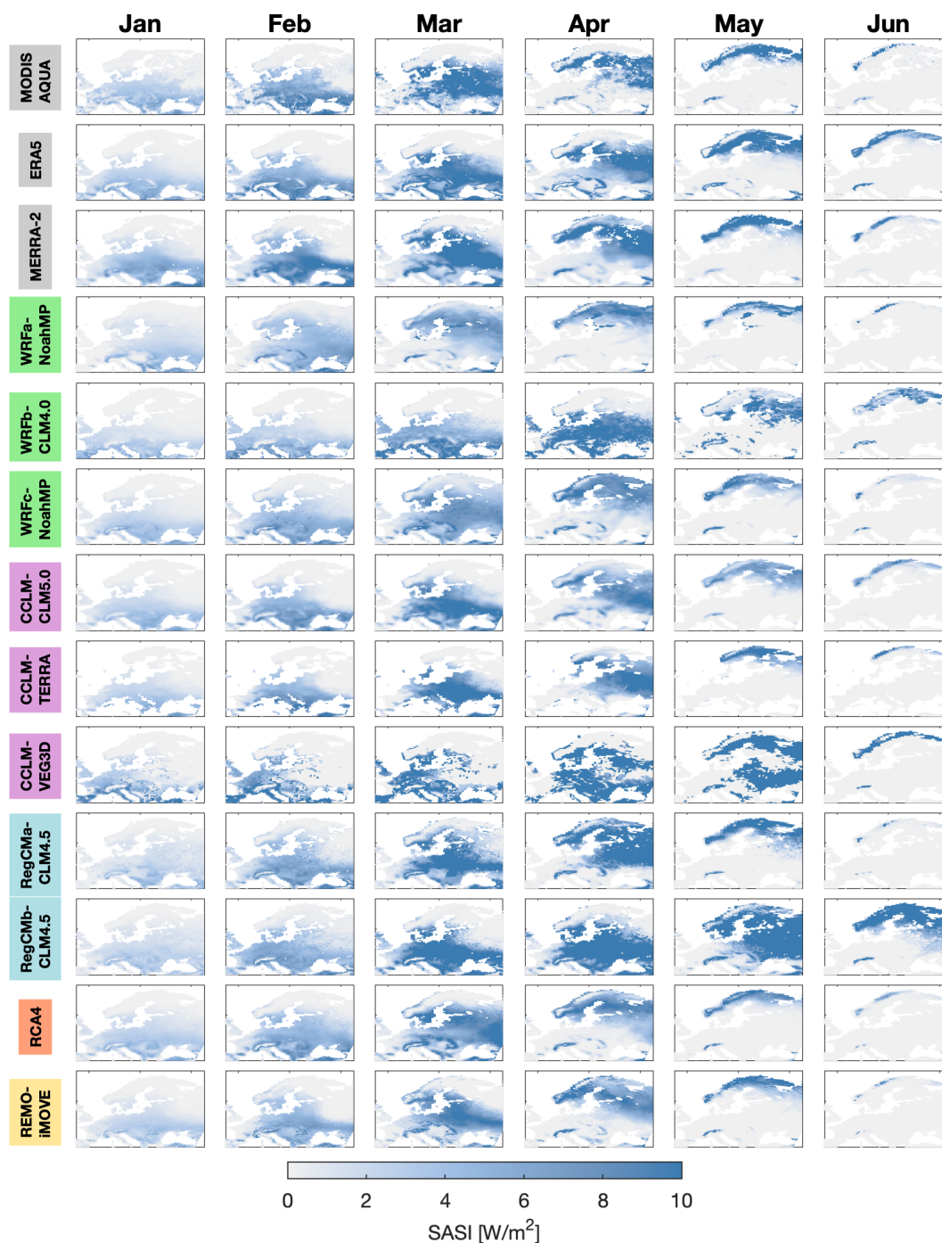
Figure 3. Spatial maps of SASI ( \text{W m}^{-2} ) for satellite observations of MODIS-AQUA, the reanalysis of ERA5-Land and the 10 RCMs from the EVAL experiment of LUCAS from January to June, averaged over the time period 1986–2015.
