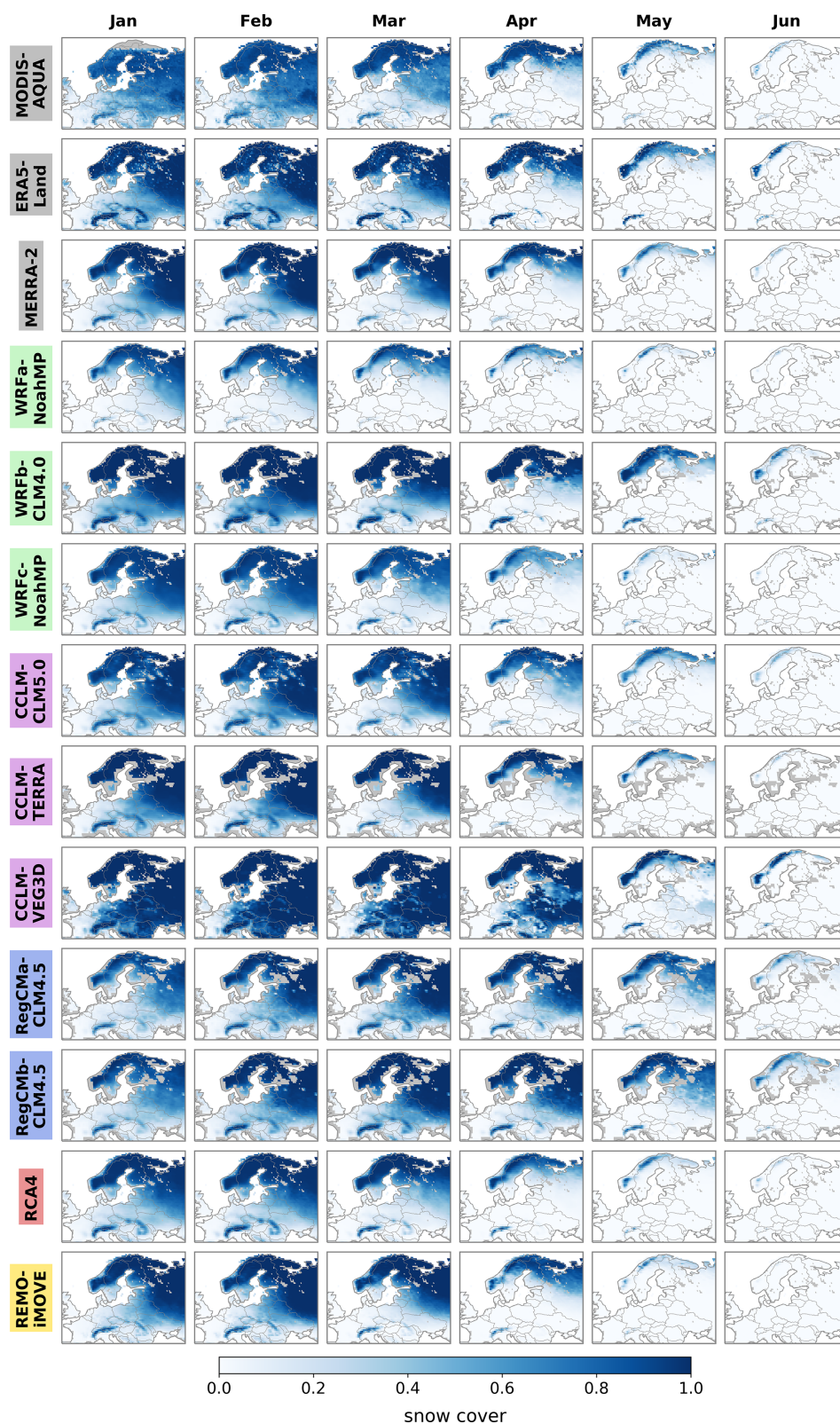
Figure 2. Spatial maps of snow cover for the satellite observations of MODIS-AQUA, the reanalyses of ERA5-Land and MERRA2, and the 10 RCMs from the EVAL experiment of LUCAS. Data show monthly averages from January to June over the period 1986–2015 for models and reanalyses and over 2003–2015 for satellite observations. See Fig. S2 in the Supplement for the same figure will all datasets averaged over the time period 2003–2015.
