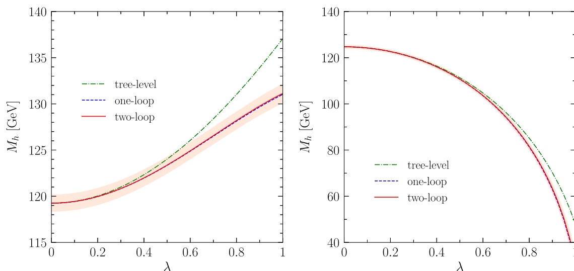
Fig. 1 Higgs-mass prediction as a function of \lambda , for \tan\beta = 3 (left) or \tan\beta = 5 (right), in the NMSSM scenario described in the text. The three lines in each plot correspond to different accuracies of the
