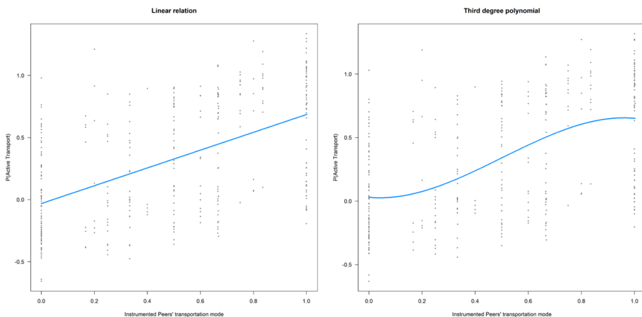
Figure 2: Assessment of the linearity of endogenous peer effects in the complete model
