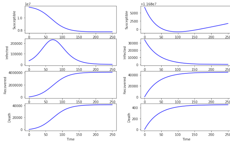
Figure 3: Dynamics of state variables per unit of time in two cases: without any control measures 1 - u_1 = u_2 = 0 (a)(on the left) and with optimal control pair (u_1^*, u_2^*) (b)(on the right)
