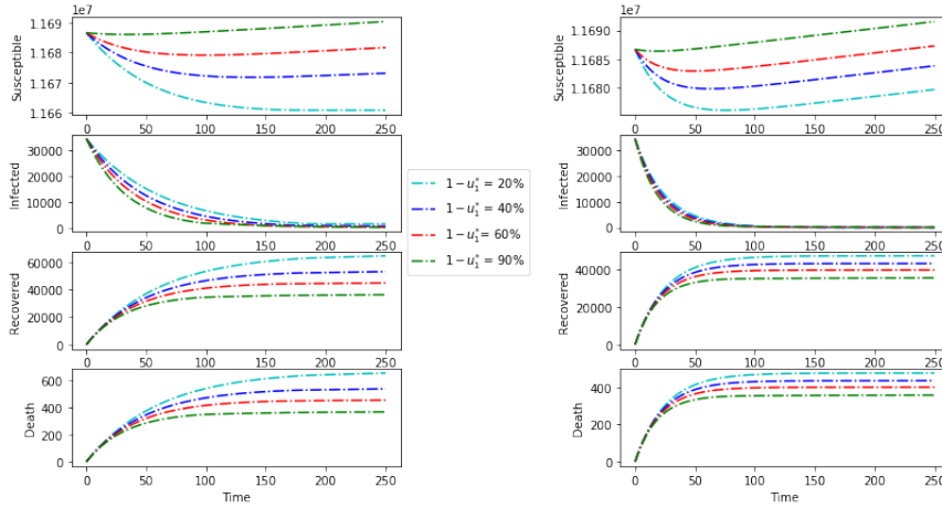
Figure 5: Simulation of SIRD model for two values of maximal screening u_2^{max} = 0.2 (on the left), and u_2^{max} = 0.5 (on the right); and four different values of mask wear 1 - u_1^{min} \in \{0.2, 0.4, 0.6, 0.9\}
