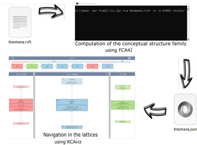
Fig. 2. Process for navigating within a Relational context family, provided as a RCFT format file, using FCA4J and RCAviz.
