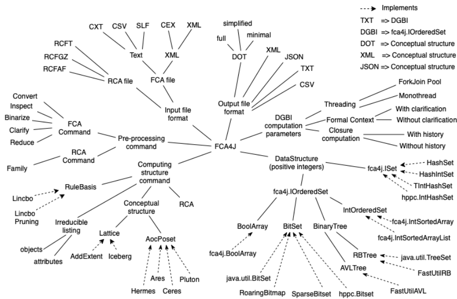
Fig. 1. An overview of all features of FCA4J
