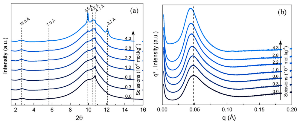
Fig. 4. Effect of chain scissions on the PEBA morphology: (a) WAXS and (b) SAXS diffractograms resulting from measurements in the quiescent state (no mechanical load applied) at room temperature.
