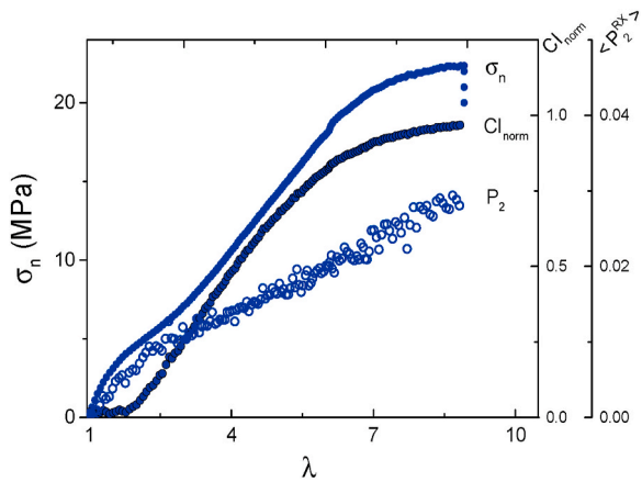
Fig. 8. Mechanical and structural changes under stretch of the PEBA sample presenting 1.0 \times 10^{-2} \text{ mol kg}^{-1} scissions induced by immersion at 80^\circ\text{C} (sample arbitrarily chosen as representative). The nominal stress \sigma_n , the normalized crystallinity index CI_{norm} , and the amorphous phase orientation parameter P_2^{RX} are superimposed to highlight structural changes along with their impact on the mechanical behaviour of the PEBA. Corresponding in situ WAXS patterns from which CI_{norm} and P_2^{RX} are determined are presented in Fig. 7.
