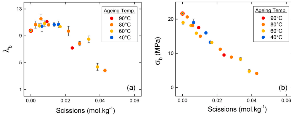
Fig. 6. Effect of chain scissions induced by immersion at different temperatures on the PEBA's (a) elongation at break and (b) nominal stress at break.
