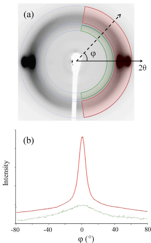
Fig. 2. (a) Diffraction pattern of a stretched sample with the two integration areas, one including the diffraction lobes and the other including a pure amorphous phase. In (b) the corresponding diffractograms are plotted, resulting from the radial integration in the respective areas.
