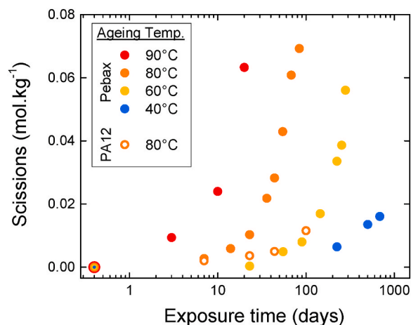
Fig. 3. Chain scission kinetics of the PEBA and the PA12 homopolymer constituting PEBA's hard segments aged at different temperatures in water.
