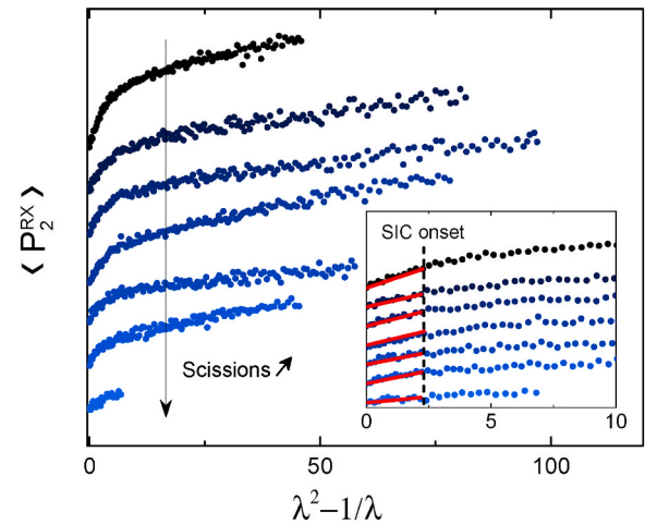
Fig. 10. Effect of scissions induced by immersion at 80^\circ\text{C} on the soft segment orientation behaviour of the PEBA. The P_2^{RX} slope was determined for 1 < \lambda < \lambda_{onset-min} , \lambda_{onset-min} being the smallest \lambda_{onset} measured (all samples considered).
