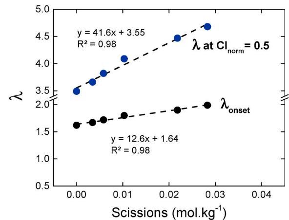
Fig. 11. Effect of chain scission, on the strain-induced crystallization onset and on the elongation required to reach a normalized crystallinity index of 0.5. Data presented here correspond to samples immersed at 80^\circ\text{C} .
