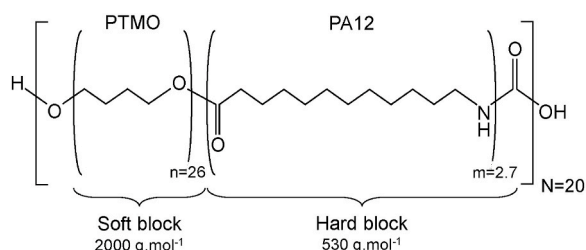
Fig. 1. Pebax® 2533 chemical structure and composition.
