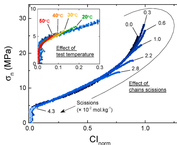
Fig. 12. Master curve between nominal stress and normalized crystallinity index of the PEBA presenting varying scission levels induced by immersion at 80 °C. Unaltered samples (not subjected to any scissions) were also tested at different temperatures.
