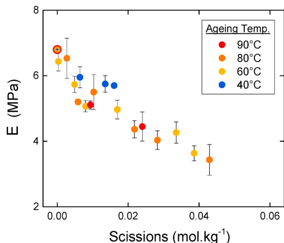
Fig. 5. Change in the PEBA modulus with chain scissions induced by hydrolysis. The tensile modulus E is defined as the slope for 1 < \lambda < 1.2 .
