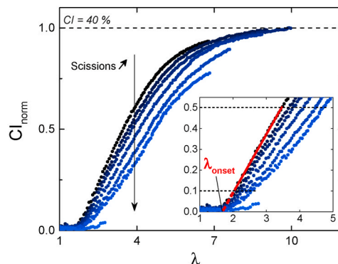
Fig. 9. Effect of scissions induced by immersion at 80^\circ\text{C} on the stress and crystallinity of the PEBA. Stars (*) on the \sigma_n - \lambda curves indicate that failure was not reached for samples subjected to none and 0.3 \times 10^{-2} \text{ mol kg}^{-1} scissions, due to slippage of the specimen out of clamps. All crystallinity index data were normalized to the highest CI value reached; all samples considered. The SIC onset was determined as the intersection of the x-axis with the CI_{norm} - \lambda curve linear fit for 0.1 < CI_{norm} < 0.5 .
