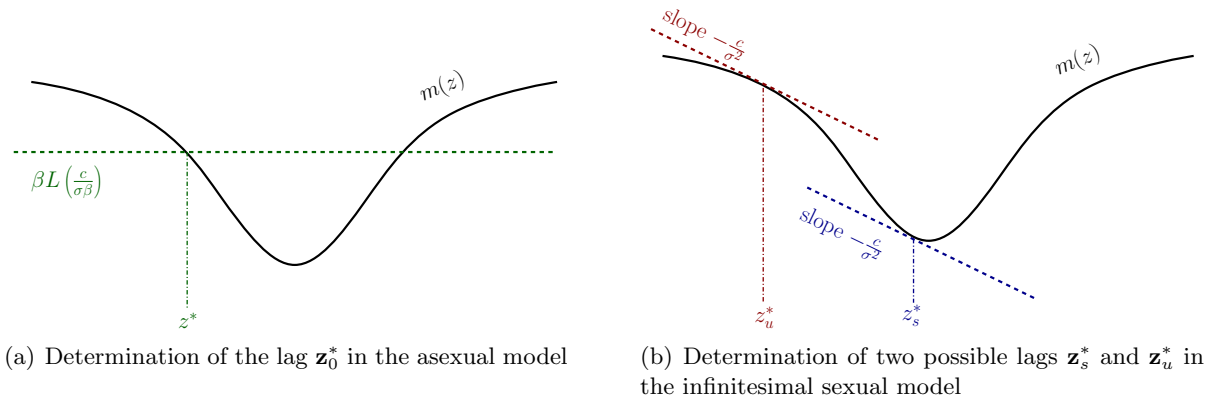
Figure 4: Graphical illustration of the two ways to characterize the evolutionary lag \mathbf{z}^* (in original units). (a) In the asexual model, the evolutionary lag is found where the mortality rate \mathbf{m} equals a specific value \beta L(\frac{c}{\sigma\beta}) . In this case we only have one possible lag \mathbf{z}^* because \mathbf{m}'(\mathbf{z}^*) and c should have opposite signs. (b) In the sexual infinitesimal model, the evolutionary lag \mathbf{z}^* is found where the selection gradient \mathbf{m}' equals a specific value \frac{-c}{\sigma^2} . In this case, we may obtain two possible values, a stable point \mathbf{z}_s^* in the convex part of \mathbf{m} and an unstable point \mathbf{z}_u^* in its concave part.
