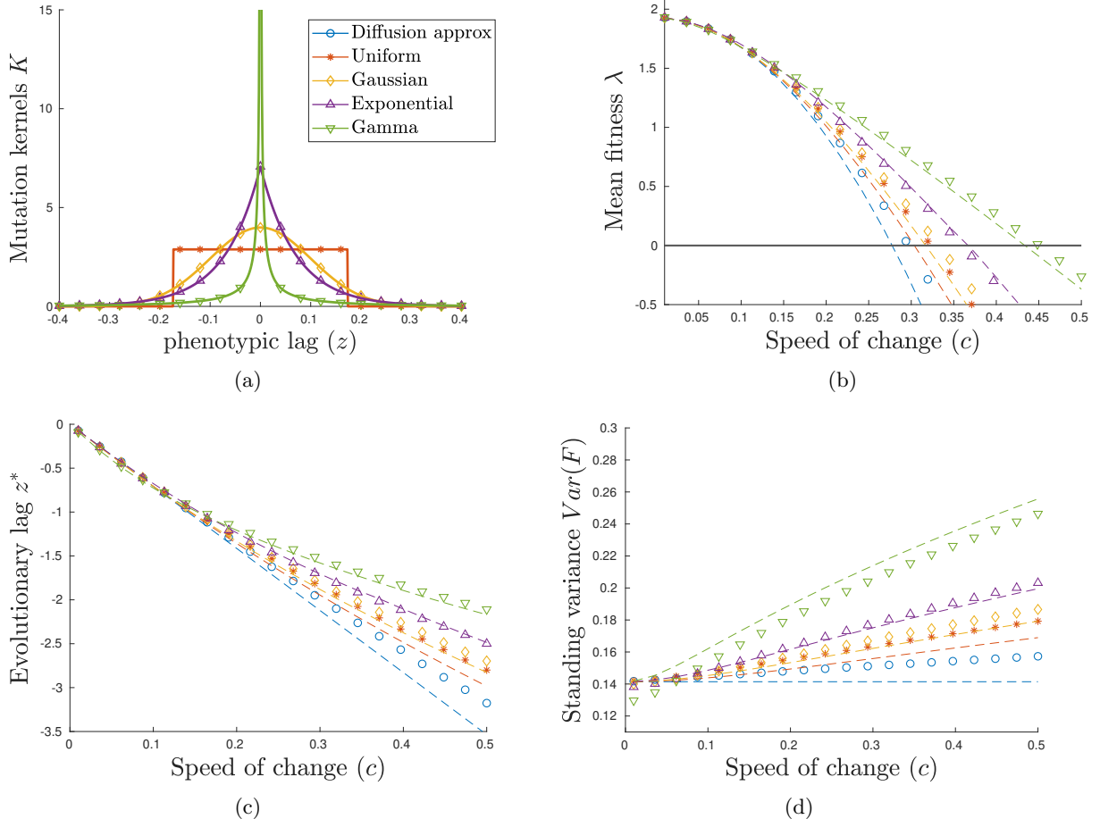
Figure 2: Influence of the mutational kernel K , described in panel (a), on (b) the mean fitness \lambda , (c) the evolutionary lag z^* and (d) the standing phenotypic variance \text{Var}(F) at equilibrium in an environment changing at rate c ranging in (0, 0.5) . We compare the diffusion approximation (blue curves) with four different mutation kernels with the same variance \sigma = 0.1 : the Uniform distribution (red curves), the Gaussian distribution (orange curves), Exponential distribution (purple curves) and Gamma distribution (green curves). Other parameters are: \alpha = 1 ; \beta = 2 . For each case we compare our analytical results (dashed lines) with the simulation results (marked symbol).
