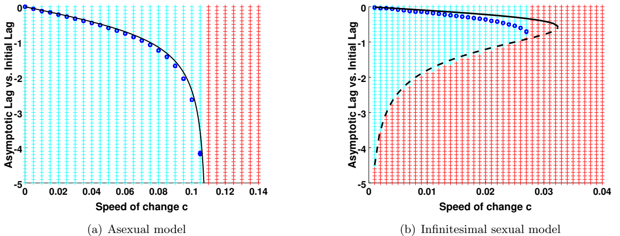
Figure 5: Effect of the mean initial lag in the persistence of the population with various rates of environmental change \mathbf{c} . We compute numerically, the solutions of the time-dependent problem (2.3) with Gaussian initial conditions centered on various evolutionary lags \mathbf{z}_{init}^* , depicted by crosses in the figures. We repeated this exploration for various speeds \mathbf{c} ranging in (0, 1.5 \mathbf{c}_{tip}^*) . For each case, we plot the evolutionary lag z^* at the final time of computations (blue circles) and the analytical evolutionary lags given by the first line of Table 2 (black lines): the plain lines corresponds to the stable trait ( z^* in asexual model and z_s^* in infinitesimal sexual model) while the dashed lines corresponds to the unstable trait z_u^* occurring in the infinitesimal sexual model. The light blue crosses correspond to initial data such that the final evolutionary lag is finite while the red crosses correspond to initial data such that the final evolutionary lag diverges. In the asexual simulations, the mutation kernel is Gaussian.
