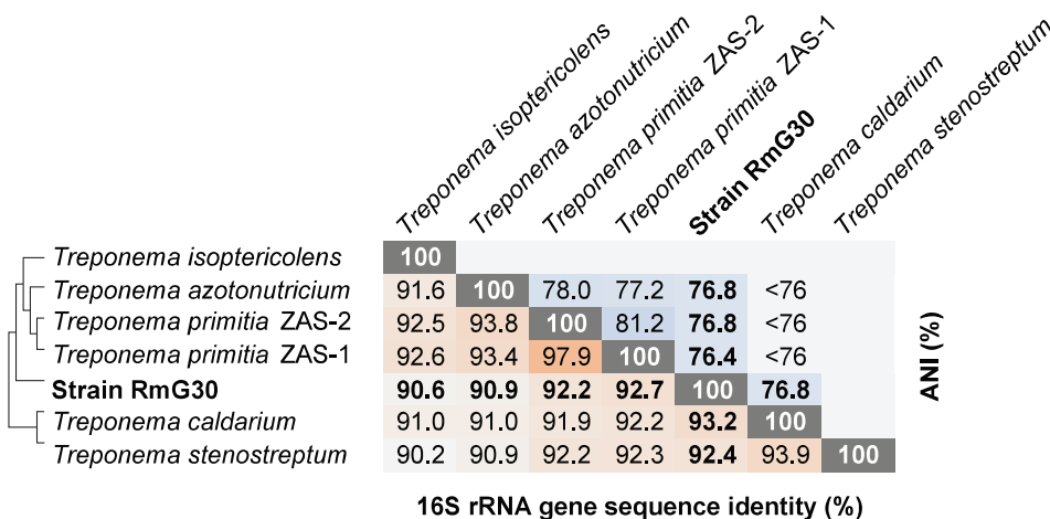
Fig 4. Pairwise comparison of sequence identity of the 16S rRNA genes and average nucleotide identity (ANI) of the genomes between strain RmG30 and its relatives in the proposed family ‘ Termitinemataceae ’. The phylogenetic relationship was taken from Fig. 2. The colour depth of each cell was adjusted according to the respective value. ANI values <76% are below the cut-off of the FastANI tool. [Color figure can be viewed at wileyonlinelibrary.com ]
